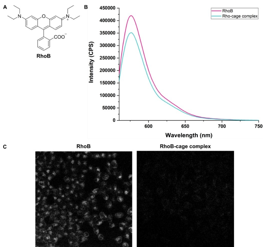
Figure 3. A) Structure of RhoB. B) Emission spectra of a 1 \mu M solution of RhoB and a 1 \mu M solution of RhoB-cage complex in water. C) Confocal microscopy images of HeLa cells incubated with a 500 nM solution of RhoB or RhoB-cage complex.
