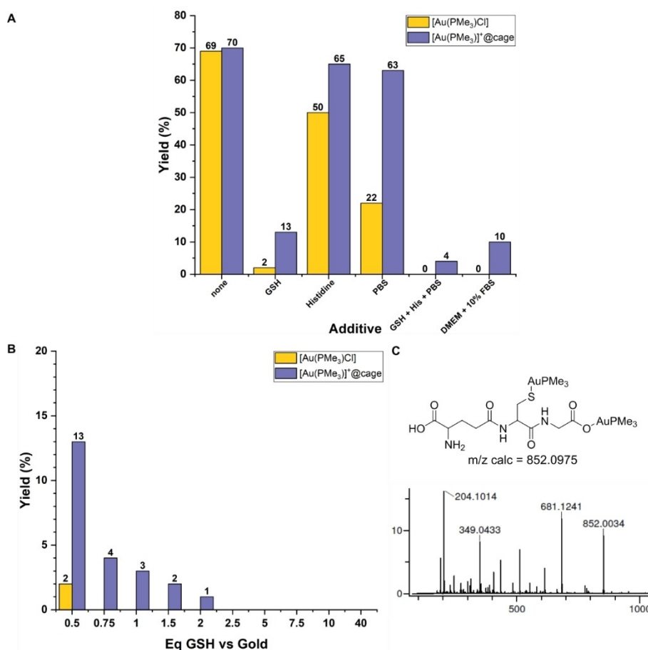
Figure 4. A) Yields of product 2 after Catalysis of substrate 1 with free [\text{Au}(\text{PMe}_3)\text{Cl}] and encapsulated [\text{Au}(\text{PMe}_3)]^+ \text{Cage} in the presence of biological additives. B) Yields of product 2 after catalysis of substrate 1 with free and encapsulated catalyst in the presence of increasing equivalents of GSH. C) ESI- HRMS spectrum (positive mode) of the catalysis reaction mixture in the presence of 0.5 equivalents of GSH with respect to gold.
