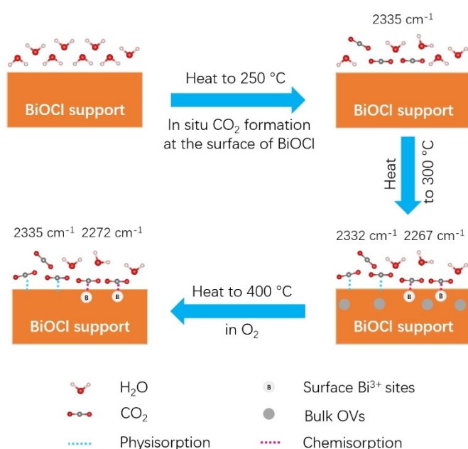
Figure 10. Proposed schematic mechanism of BiOCl OV formation based on in-situ DRIFTS results in Figure 9.
