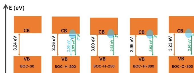
Figure 8. Defect state positions of BiOCl samples, calculated from bandgap and photoluminescence spectra.
