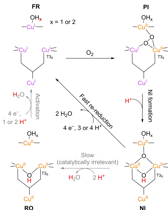
Scheme 2. General catalytic cycle for ORR in the TNC. His/Cys ligands are shown in a skeleton-like fashion for brevity. Arrows indicated in grey are catalytically less relevant. The reaction of the resting oxidized (RO) to the fully reduced (FR) state is an activation step. The actual ORR cycle starts when O_2 diffuses into the TNC to form the peroxide intermediate (PI). PI quickly decays to the native intermediate (NI) in 2 double IET steps, in which a proton is transferred most likely from the carboxylic acid moiety of the T3 Glu/Asp residue. NI has the same oxidation state as RO. The ORR cycle is closed by the proton-coupled re-reduction of the NI, consuming four equivalents of oxidizing substrate under excretion of 2 equivalents of water. NI to RO is a deactivation step, which becomes significant only when no oxidizing substrate and/or O_2 is present anymore. This mechanism is based on a catalytic cycle provided by Jones and Solomon 2015. [21b]
