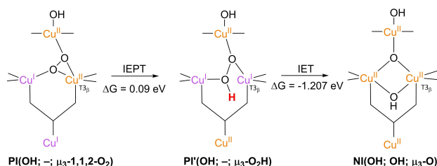
Scheme 11. PI decay as proposed by Li et al. 2015. [46c] In this work, both T3 Glu/Asp and T2 Asp were kept deprotonated and the T2 WD ligand was claimed to be OH throughout the catalytic cycle. The proton in the IEPT step is delivered from an Asp residue on the surface of the protein which is not involved in any H-bonding network. This residue was chosen as proton donor/acceptor in this work for technical reasons. Note that the oxidation states of each of the Cu ions has been assigned somewhat arbitrarily in PI, as the authors indicated these to be hard to identify in some intermediates. For PI', a T2 Cu II state could be identified, rendering the T3 Cu ions in the reduced state. Free energies were obtained using QTCP-2QM calculations with B3LYP-D3/def2-TZVPD as the final combination of functional/basis set. These QM/MM calculations were carried out in a 38 Å radius spherical system of explicit H 2 O molecules. Contributions of dissociated H 2 O to reaction free energies were approximated by modeling the molecule in a dielectric continuum with \epsilon = 80 , using a B3LYP functional and a def2-TZVP basis set.
