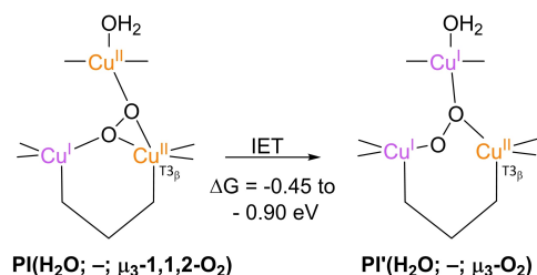
Scheme 10. Energetics of the IET reaction converting PI to PI' according to Hu et al. 2011. The structure of PI (H 2 O; −; μ 3 -1,1,2-O 2 ) was obtained from Yoon and Solomon 2007, and the structure of PI' (H 2 O; −; μ 3 -O 2 ) was based on a PI' structure proposed by Rulišek et al. 2005. [31b,38] Cu oxidation states are complemented from these sources as Hu et al. did not specify these in their paper. In all calculations a solvation shell of explicit H 2 O molecules was used with a radius of 38 Å. \Delta G estimates were calculated using a Perdew-Burke-Ernzerhof (PBE) functional and a def2-SVP basis set. \Delta G = -0.45 eV was calculated by QTCP-2QM methodology. \Delta G = -0.90 eV was calculated using averages of QM/MM calculations of snapshots on MD simulations of the PI and PI' structures under thermodynamic standard conditions.
