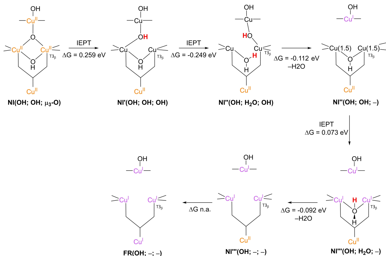
Scheme 14. The second suggested mechanism for regeneration of FR from NI. [46c] The last reductive step was not included in the simulation. Free energies were obtained using QMCP-2QM calculations with B3LYP-D3/def2-TZVPD as the final combination of functional/basis set. These QM/MM calculations were carried out in a 38 Å radius spherical system of explicit H 2 O molecules. Contributions of dissociated H 2 O to reaction free energies were approximated by modeling the molecule in a dielectric continuum with \epsilon = 80 , using a B3LYP functional and a def2-TZVP basis set.
