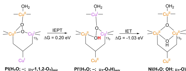
Scheme 12. Decay of PI(H 2 O; -, \mu_3 -1,1,2-O 2 ) mir to NI(H 2 O; OH; \mu_3 -O), via a PI'(H 2 O; -, \mu_3 -O 2 H) mir intermediate as obtained by Siegbahn 2020. [63b] In his model, the proton in the IEPT step was donated by solvent H 2 O at pH 7. The T2 Asp was stated explicitly to be deprotonated. T3 Glu/Asp was not considered in this simulation. The T2 WD ligand was considered to be H 2 O throughout the entire cycle. Note that in this work the oxidation state of the Cu ions in the PI and PI' structures were not specified. Free energies were calculated using DFT with a B3LYP-D3 functional with 10% exact exchange, an LAV3P* basis set for the Cu ions and a cc-pvtz(f) basis set for all other atoms. Solvation effects were modeled in a dielectric continuum with \epsilon = 4.0 . The energies were calibrated to experimentally obtained data for ORR at pH 7 and a T1 Cu II redox potential for the MCO in question.
