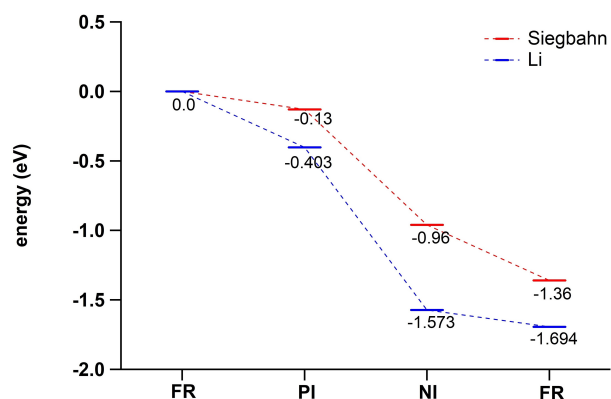
Figure 11. Free energy landscape of the Lacasse key intermediates FR , PI and NI based on the work of Siegbahn (red, 10% HF) and Li et al. at pH 7. Energies are scaled versus the reduction potential of 0.46 V for Cu T1.
