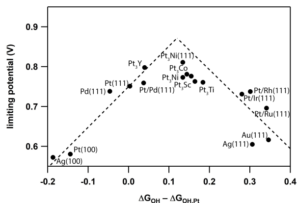
Figure 1. Volcano plot showing the experimental ORR potentials for a series of heterogeneous catalysts, showing that in the most optimized form the ORR reaction proceeds with a ~400 mV overpotential. Data in the figure are based on literature. [7b]
