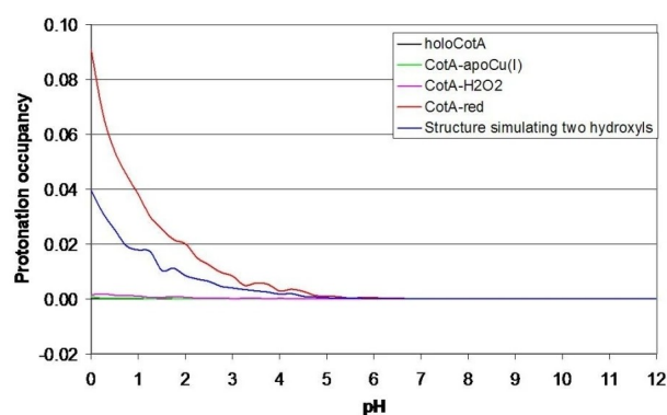
Figure 10. Proton-inactivity of T2 Asp as observed in simulated pH titrations of this residue in various CotA structures. The red curve belongs to CotA in the FR state; the curve in magenta resembles the PI structure. Reproduced from Ref. [34e]. Copyright 2010, with permission from Springer nature.
