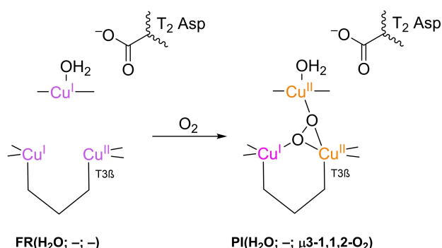
Scheme 4. Formation of PI according to Solomon et al. (2010). O 2 coordinates along the T2-T3 β edge of the TNC, as the Cu II ions along this edge have a lower tendency to be reduced, due to the negative charge of the carboxylate, as was predicted by in vacuo DFT simulations of the PI geometry. [38–39] The T2 WD ligand is included as H 2 O in accordance with the way it was simulated by Yoon and Solomon in 2007. [38] Note that in the simulation T2 Asp was represented by a formate group.
