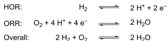
Scheme 1. Combustion of \text{H}_2 consisting of the anodic hydrogen oxidation reaction (HOR) and the cathodic oxygen reduction reaction (ORR). The thermodynamic standard potential is 1.23 V vs. NHE
