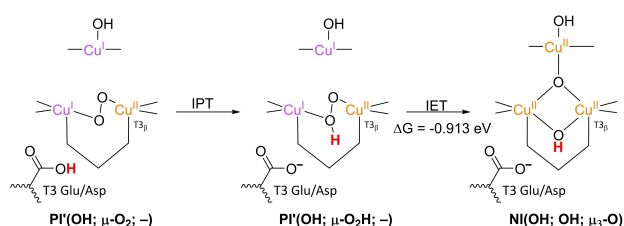
Scheme 9. Decay of PI' to NI according to Srnc et al. 2011. [69] Preliminary calculations indicated a pK_a increase of the peroxide ligand by 11 pH units over the course of the PI → PI' reaction. Together with the abovementioned experimentally observed pH-dependence of PI decay to NI , this motivated the authors to propose an IPT step prior to the actual O–O bond cleavage via the IET step. The authors did not perform any explicit I(E)PT simulation, and the T2 WD ligand always remained in the same protonation state (either H 2 O or OH − ). With OH − , the IET step was found to be slightly more favorable than with H 2 O). The final value of the IET electronic energy was calculated using QM/MM DFT on single-points of geometry optimized structures with a B3LYP functional and a def2-TZVP basis set. The enzyme was dissolved in a sphere of explicit H 2 O molecules with a radius of 38 Å. [31b] To estimate the Gibbs reaction energy, thermal enthalpic and entropic contributions were estimated by means of a normal mode analysis of small in vacuo models of the TNC, excluding the T2 WD ligand, crystalline H 2 O and any 2 nd coordination sphere residues. The thermodynamic conditions of this analysis were pH 7, 298.15 K and 1 atm pressure. [69]
