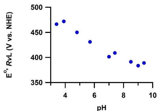
Figure 6. pH-dependence of E_{RvL,T1}^{0'} . Blue data: original values as reported by Nakamura, 1958. [27g]
