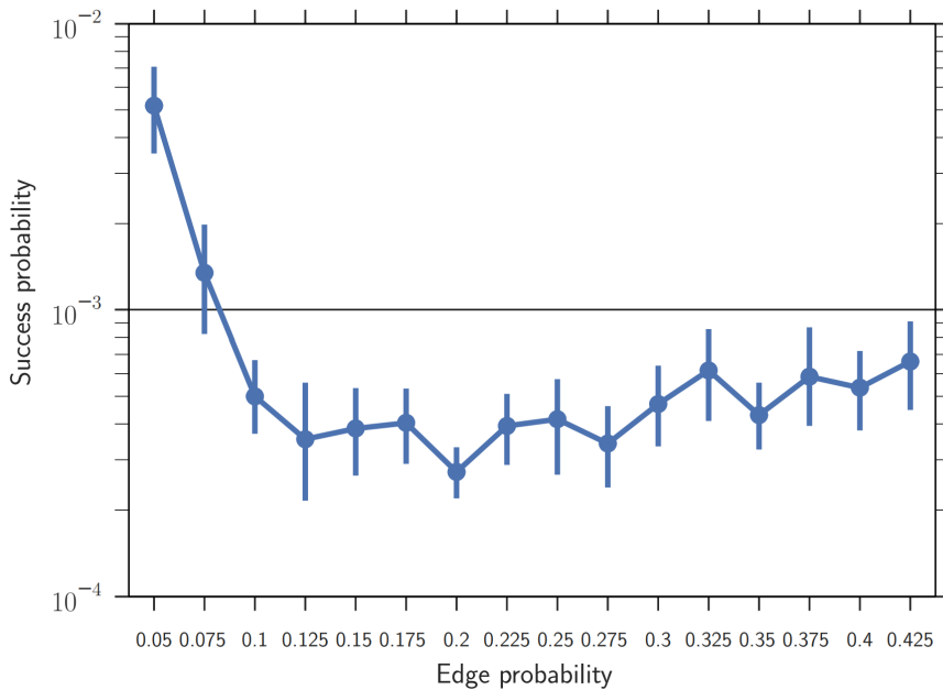
Figure 3.1: Distribution of success probabilities of the tested D-Wave 2000Q QPU as a function of edge probability p for randomly generated graphs (50 graphs at each point of p ). The maximum point of difficulty (e.g., lowest mean success probability) was observed at p = 0.2 . Error bars are bootstrapped 95% confidence intervals.
