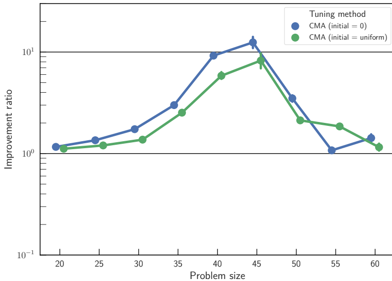
Figure 3.8: Ratio of mean success probabilities, before and after tuning, for each of the two strategies. All points are above 10^0 , and indicate an improvement in probability. The peak is observed at n = 45 for both initial settings, with an improvement of 12.4 for the null configuration and 8.2 for the uniform configuration.
