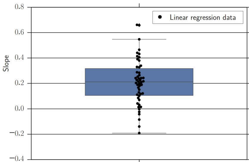
Figure 3.2: Boxplot showing the distribution of linear regression slopes of 50 MIS problems at n = 50 and p = 0.2 (25 embeddings used for each point), all solved using a D-Wave 2000Q QPU. The majority of the points lie above zero, indicating the larger embeddings cause the QPU to find worse optima.
