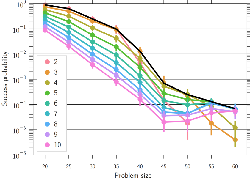
Figure 3.3: The probability of the D-Wave 2000Q QPU finding the putative optimum of each problem for different chain strengths. The black line shown is the envelope of optimal chain strengths at each problem size n . As n increased, larger magnitude chain strengths were optimal.
