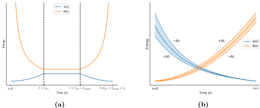
Figure 3.5: (a) Diagram of a simple reverse annealing protocol (with duration t_{\text{rev}} in reverse and t_a forward) with a pause (of duration t_{\text{pause}} ) in the middle. (b) Diagram of possible annealing schedules using an anneal offset of maximum magnitude |\Delta t_i| .
