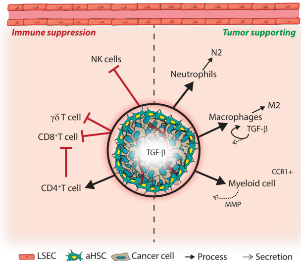
FIGURE 7 TGF- \beta secretion and signaling in liver metastases can provide protection to innate and adoptive immune responses. Transforming growth factor (TGF)- \beta secretion of tumor cells and fibroblasts, and the resulting fibrotic niche, provides a physical barrier against immune cells and triggers immune suppressive effects in immune cells. Neutrophils and macrophages could differentiate toward tumor supportive N2 and M2 type cells. Moreover, TGF- \beta secretion by macrophages further enhance immune suppression. Anti-tumor effects of Natural Killer (NK) cells can be inhibited by TGF- \beta . Tumor supporting myeloid cells derived from the bone marrow support metastasis formation and are recruited to metastases through e.g. binding of secreted C-C Motif Chemokine Ligand 15 (CCL15) to the C-C chemokine receptor type 1 (CCR1) receptor. These cells support metastasis by contributing to immune suppression and secreting matrix modulating proteins such as matrix metalloproteases (MMPs). During liver metastasis formation, the effects of cytotoxic CD8 + and \gamma\delta T cells are inhibited by TGF- \beta , through e.g. reduction of T cell infiltration or proliferation, reduced T cell activation and inhibition of cytotoxic effector proteins, while immune suppressive CD4 + regulatory T cells are stimulated
