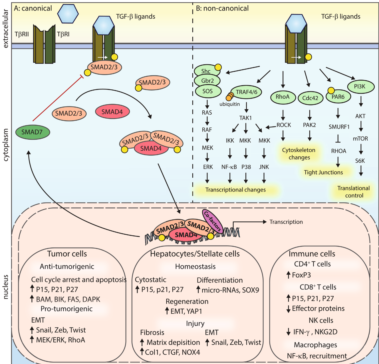
FIGURE 2 Canonical and non-canonical TGF-β signaling. Transforming growth factor (TGF)-β ligands initially bind to TGF-β receptor (TβR)II, and thereafter recruit TβRI. A heteromeric TGF-β receptor complex is formed in which the TβRII kinase transphosphorylates TβRI. A, In canonical TGF-β signaling, intracellular effectors mothers against decapentaplegic homolog (SMAD)2 and SMAD3 are phosphorylated by TβRI, which thereafter can bind to SMAD4. This complex translocates into the nucleus, and together with other co-factors, regulates the expression of TGF-β target genes in a context dependent manner. A negative feedback loop is created through induced expression of inhibitory SMAD7, which by partnering with Smad ubiquitination regulatory factor (SMURF) E3 ubiquitin ligases, targets the TβRI for ubiquitin-mediated degradation. B, Non-canonical TGF-β signaling includes multiple different signaling pathways that are not unique for TGF-β signaling, an overview is given in this figure. TGF-β can elicit different responses in different cell types, depending on the cellular context. In tumor cells, TGF-β/SMAD pathway can induce cytostatic effects through upregulation of cell cycle arrest and apoptosis genes. Pro-tumorigenic effects of TGF-β occur through SMAD-dependent upregulation of EMT transcription factors and also non-canonical signaling play a role. In hepatic and stellate cells, TGF-β can induce cytostatic effects, but also differentiation and regeneration. During injury, TGF-β signaling promotes fibrosis through e.g. matrix deposition and stimulating EMT. In immune cells, TGF-β dampens immune responses. Cytotoxic effects of CD8 + T cells and natural killer (NK) cells are repressed, while regulatory CD4 + T cells and (immune suppressive) macrophages are promoted
