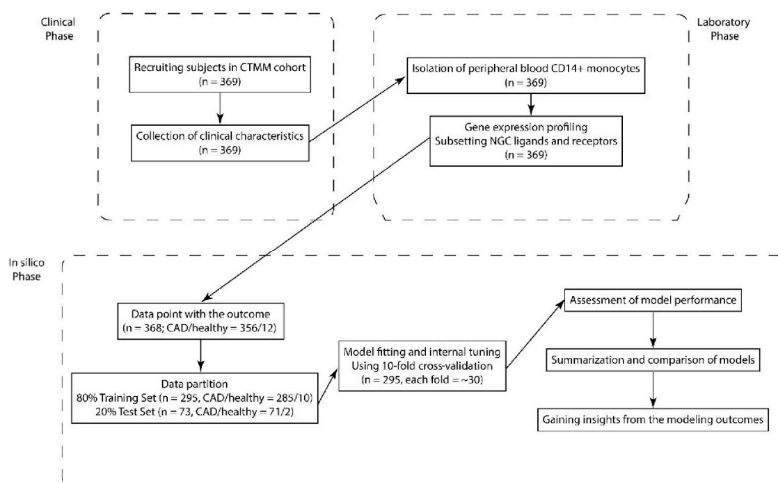
Figure 1. Flowchart of predictive modeling using neuroimmune guidance cues (NGCs). Subjects in the CIRCULATING CELLS cohort were recruited based on inclusion criteria. The clinical characteristics were collected, peripheral blood CD14-positive monocytes were isolated and their transcriptomes were profiled. The expression of NGCs was subset. The individuals were randomly assigned to the Training Set or Test Set for external assessment of the model performance. Classification models that were built on the Training Set data and model performance were internally assessed with cross-validation. Finally, we made comparisons between the models and gained insights on the choice of model and features.
