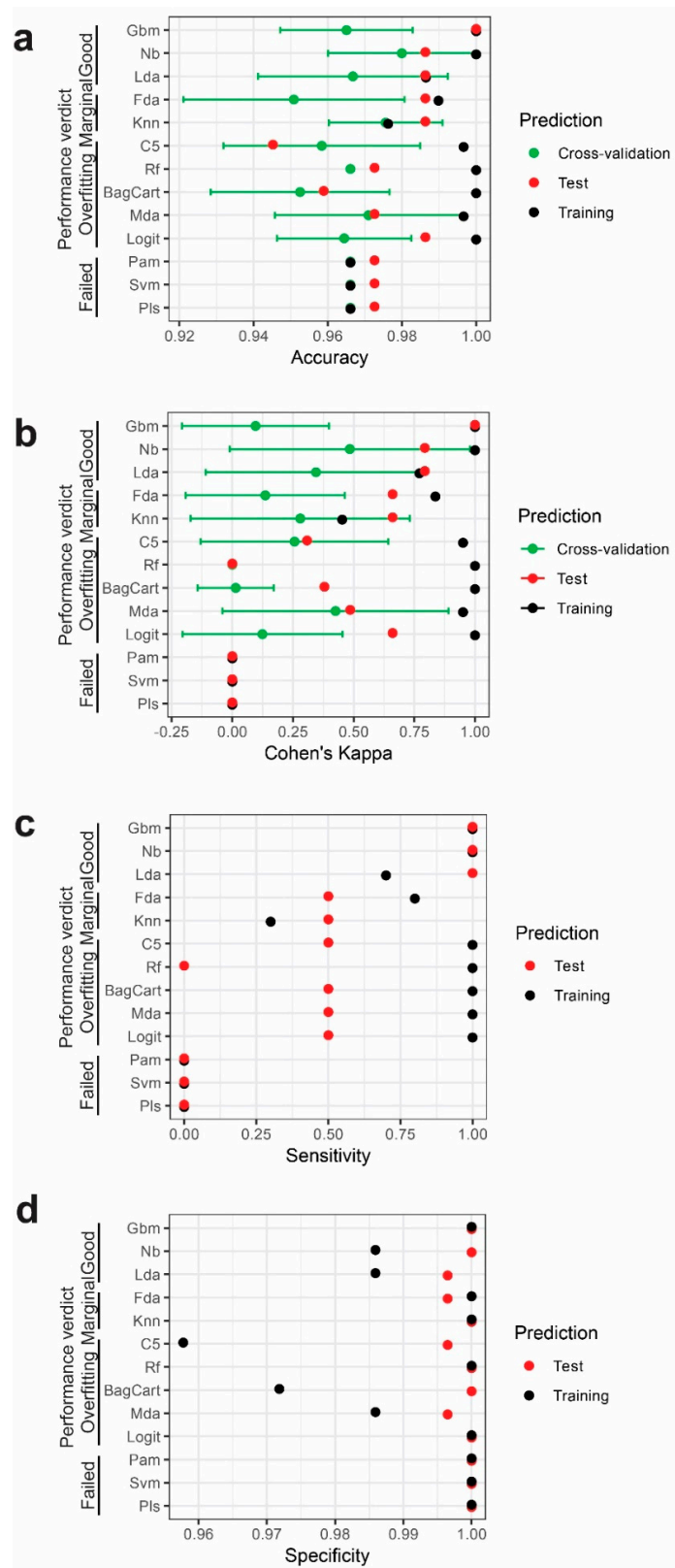
Figure 6. Model performance. (a–d) Model performance metrics—namely, accuracy (a), Cohen’s Kappa (b), sensitivity (c) and specificity (d)—were illustrated in cross-validations (green dots and error bars), Training Set (black dots) and Test Set (red dots) for all models. Models are categorized into 4 groups based on their performances.
