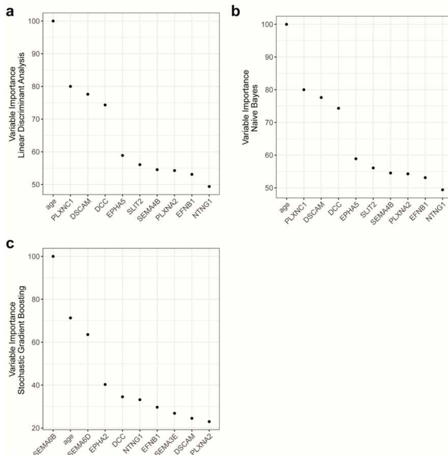
Figure 7. Variable importance of the models. (a–c) Variable importance measured in the linear discriminant analysis (a), Naïve Bayesian model (b) and stochastic gradient boost model (c). The importance of the most important feature was scaled to 100.
