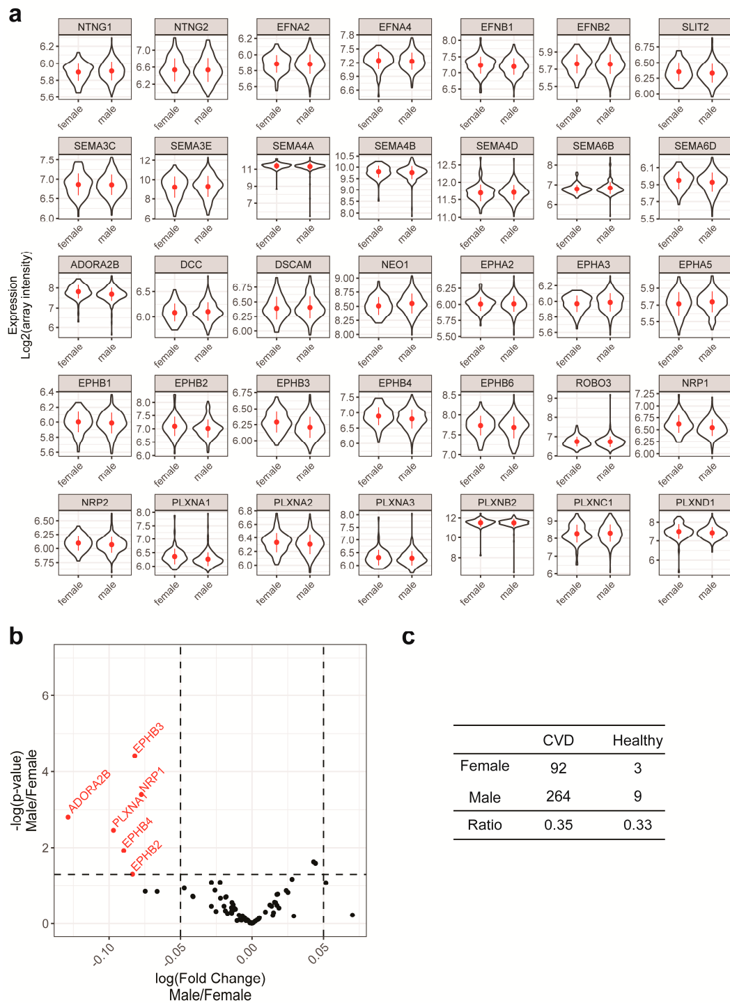
Figure 5. Inspection of the influence of sex as a potential confounding factor. (a) Violin plots to show the distribution of expressions of selected NGCs in males and females. To be noticed is that distributions of selected NGC expressions are similar between sexes. (b) A volcano plot was made showing the fold change and the significance of differences in a 2 mean Student’s t -tests between NGC expressions in males and females. NGCs with significant differences ( p < 0.05 ) were labeled with gene names and red color. (c) Contingency table showing that the ratio of sexes is not biased in relation to the outcomes.
