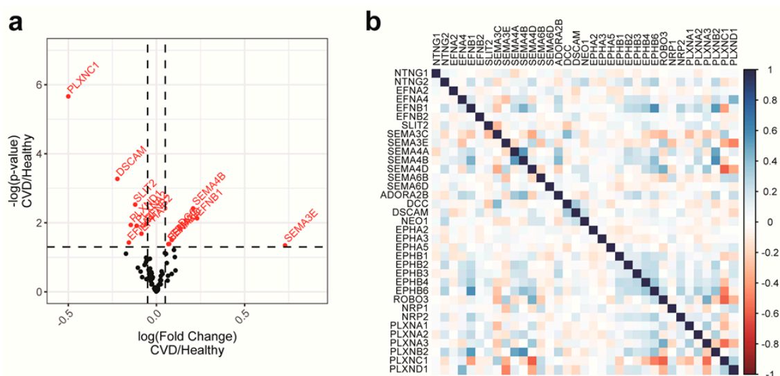
Figure 3. Univariate correlation of NGC expressions with disease phenotypes and pairwise correlations of NGC expressions. (a) Volcano plot showing the fold changes and the significance of difference in the 2 mean Student's t -tests between NGC expressions in CVD patients and healthy individuals. NGCs with significant differences ( p < 0.05 ) are labeled with gene names and red color. For most NGCs, the univariate correlation determined by the 2 mean Student's t -tests with the outcomes is minimal. (b) Pairwise covariances of NGC expressions were illustrated in the heatmap to examine the between-feature correlations. Blue color indicates a positive correlation, whereas red color indicates a negative correlation. There are no absolute pairwise covariances higher than 0.75, the common cutoff for highly correlated features.
