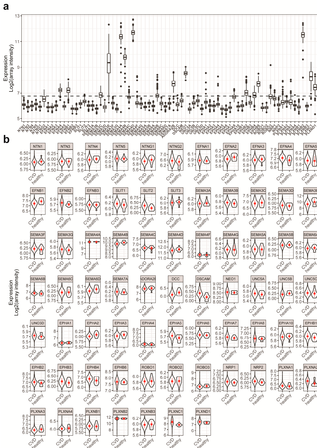
Figure 2. NGC expressions in patients and healthy subjects. (a) Box plots with quartiles were created using NGC expressions from all individuals. Baseline signal of the platform (6.75) was indicated with the dashed line. (b) Violin plots of all NGC expressions were created for cardiovascular disease (CVD) patients and healthy individuals. The violin shapes represent the density distribution of NGC expressions in the groups. The NGC expressions of CVD patients overlap with those of healthy individuals. Due to the small number of healthy individuals, their NGC expressions were sometimes not normally distributed.
