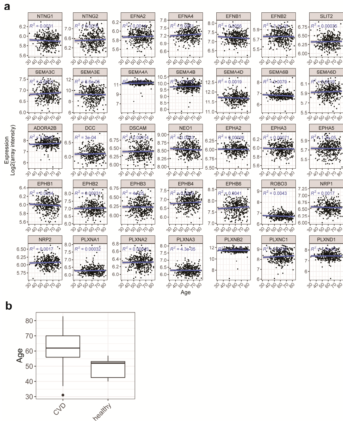
Figure 4. Influence of age as a potential confounding factor. (a) Scatter plots of expressions of selected NGCs in relation to age were made to show the influence of age on NGC expressions. Linear regressions were done with age being the dependent variable providing the fitted trend line (blue line), the 95% confidence interval of the trend (gray area) and the regression R-squared. Correlations of NGC expressions and age are minimal, as indicated by the R-squared values. (b) Boxplot of age distribution in CVD patients and healthy individuals. Young age dominates in the healthy individuals.
