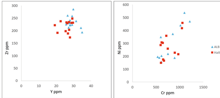
Figure 4. Body chemical composition from ICP-OES analysis. Biplots of Zr vs Y (ppm) and Ni vs Cr (ppm) of the taches noires retrieved in Haiti and the reference samples from Albisola
