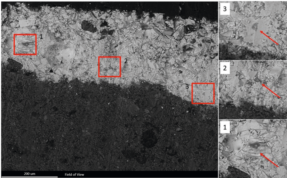
Figure 7. BSE images of the glaze in sample GD316-2. Relict iron-oxide inclusions, indicated with an arrow, are visibly dispersed in the glaze.
