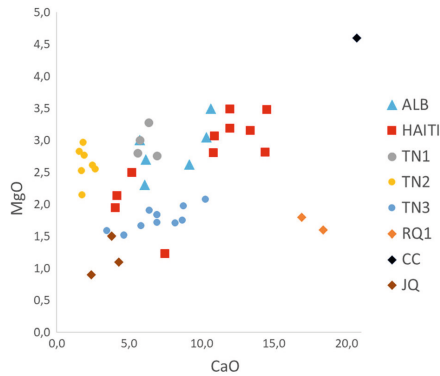
Figure 5. SEM-EDS analysis of the ceramic materials. Biplot of CaO (wt%) and MgO (wt%) for the taches noires wares retrieved in Haiti and the reference samples from Albisola (ALB and TN1) and the previous analysis of taches noires ware from Barcelona (TN2 and TN3) (Di Febo et al. 2018) and production from Provence: Roquefeuille (RQ1), Cucuron (CC) and Jouques (JQ) (Capelli et al. 2017)
