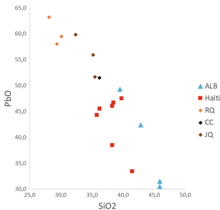
Figure 6. Glaze chemical composition from SEM-EDS analysis. Biplot of SiO 2 (wt%) and PbO (wt%) of the glaze of taches noires wares retrieved in Haiti and the reference samples from Albisola (ALB) and samples from Provence: Roquefeuille (RQ), Cucuron (CC) and Jouques (JQ) analysed by Capelli et al. (2017)
