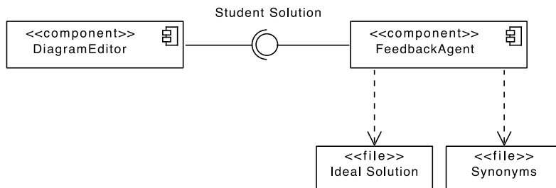
Figure 10.2: The high level overview of WebUML including the feedback agent
