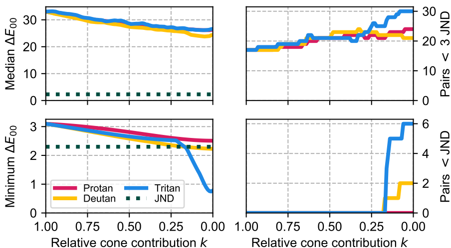
Figure 2.5: Discriminability of Forel-Ule colours. The median and minimum (left) \Delta E_{00} difference between FU colour pairs, and the number of pairs within 3 and 1 JND (right), are shown as a function of the relative cone contribution k . k ranges from 1 (full colour vision) to 0 (dichromacy), with intermediate values representing partial colour blindness (anomalous trichromacy). Pairs with \Delta E_{00} < 1 JND are fully indistinguishable, pairs with <3 JND are difficult to distinguish (Section 2.3.2).
