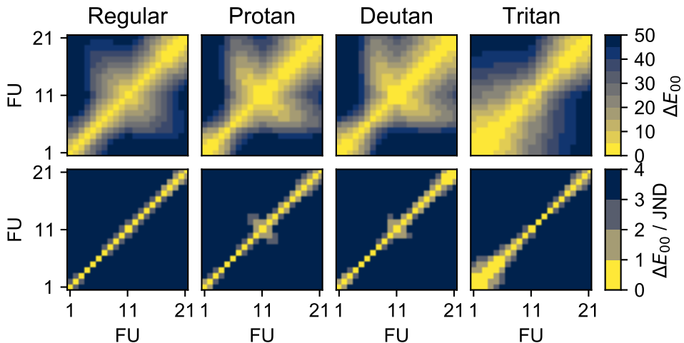
Figure 2.4: Confusion matrices for regular and deficient colour vision. The top panels show the full range of \Delta E_{00} , while the bottom panels have a narrower colour bar, in units of just-noticeable difference (JND, \Delta E_{00} = 2.3 ). Even with regular vision, some pairs of FU colours are difficult to distinguish ( \Delta E_{00} \leq 3 JND) Protan and deutan primarily decrease the discriminability of the middle (green) and high (brown) colours, while tritan primarily affects the low (blue) colours, as expected.
