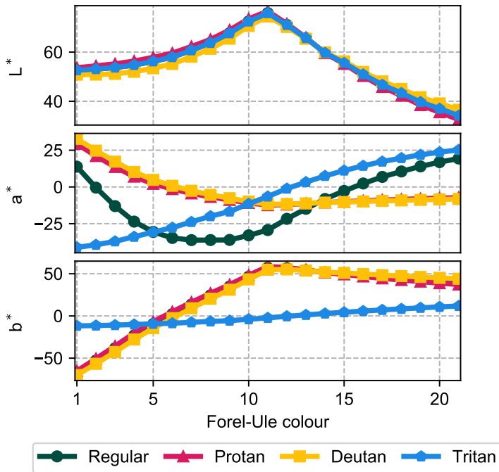
Figure 2.3: Forel-Ule colours in CIE Lab space. Both regular and deficient vision are included. Regular vision is hidden in the top and bottom panels behind protan and deutan. These affect the a^* (green-red) coordinate the most while tritan affects b^* (blue-yellow) the most. None of the deficiencies significantly affect L^* (lightness).
