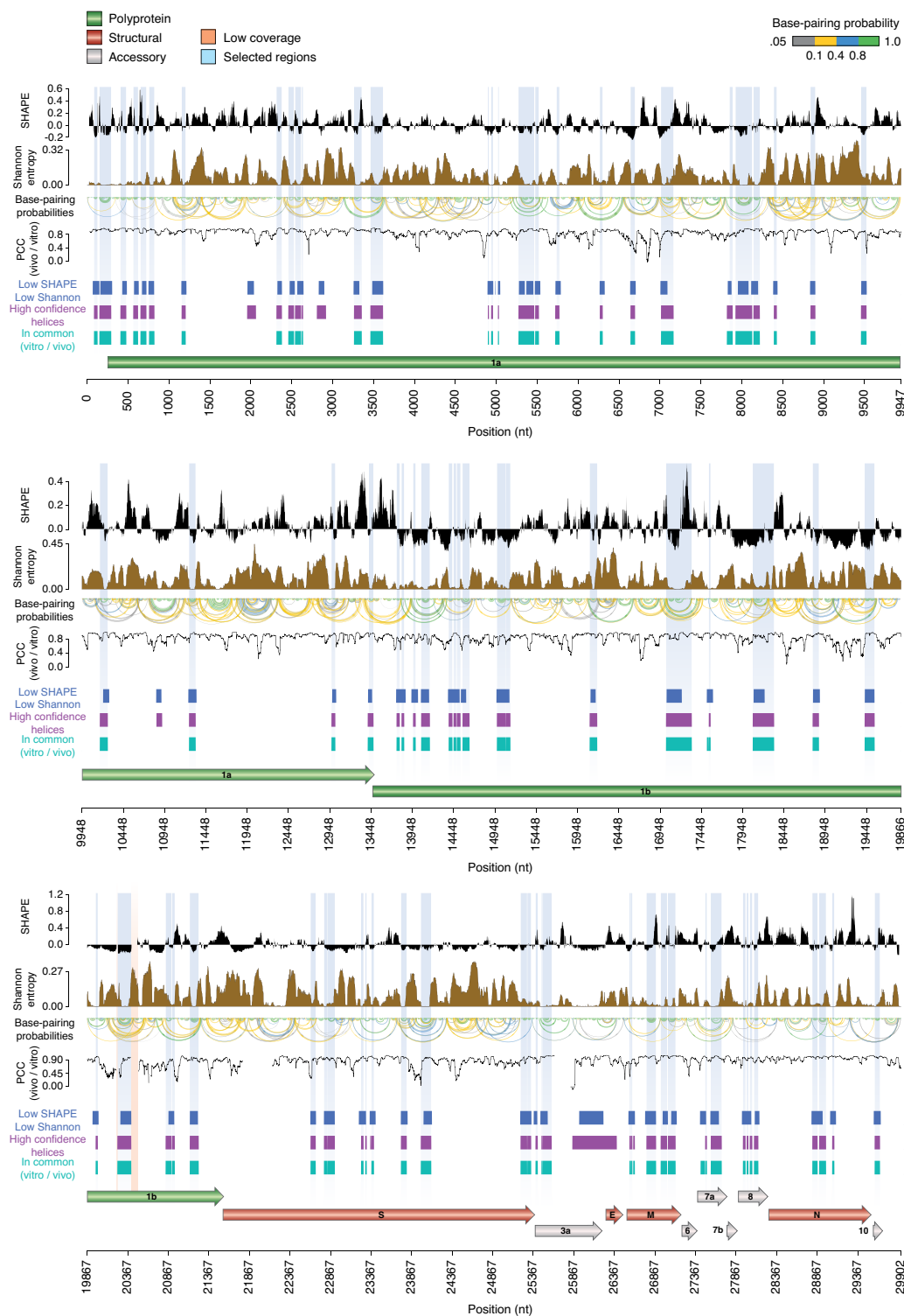
Figure 4. Structure map of the full SARS-CoV-2 genome in vivo . Map of the SARS-CoV-2 genome depicting (top to bottom): median SHAPE reactivity (in 50 nt centered widows, with respect to the median reactivity across the whole genome), Shannon entropy, base-pairing probabilities, Pearson correlation coefficient (in 50 nt centered windows; PCC) between in vitro and in vivo SHAPE data, set of low SHAPE – low Shannon under both in vitro and in vivo conditions (blue), set of helices coherently predicted independently of the window size employed (3000, 5000 or 10 000 nt; magenta), set of helices coherently predicted under both in vitro and in vivo conditions (aqua green). Selected structure elements are marked in light blue. Two short regions of low sequencing coverage are marked in red.
