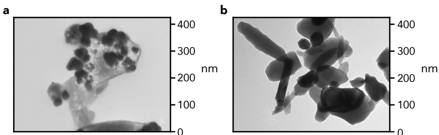
Figure 4.1: Transmission electron microscope images of nAg and nZnO particles at 60k and 50k magnification respectively.
