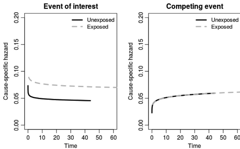
FIGURE 2 Cause-specific Weibull hazard rates with a direct effect of exposure due to an increased hazard of the event of interest with exposure. The hazard of exposure was \alpha_{01} = 0.06 and time constant
