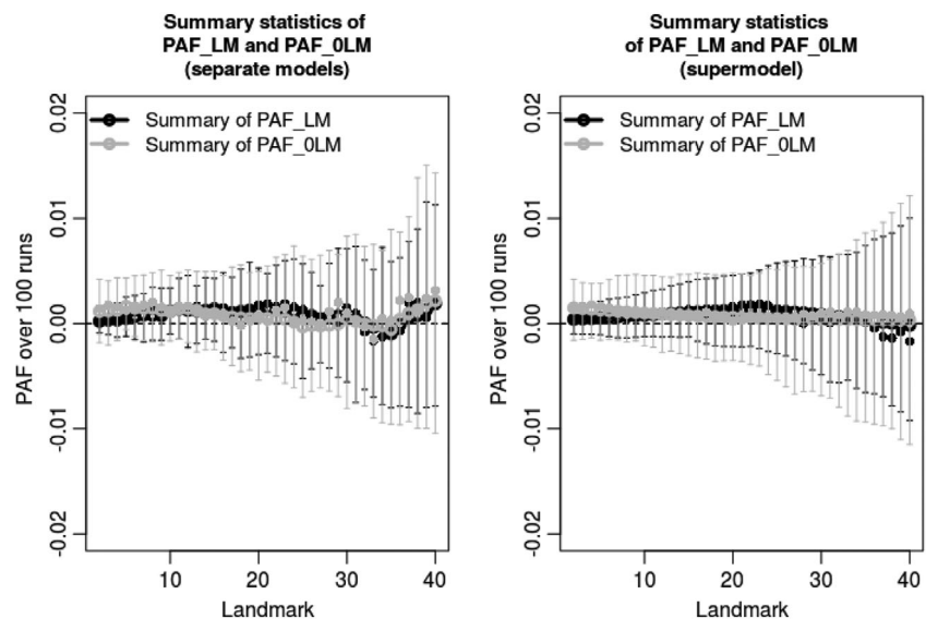
FIGURE 3 Simulation of a no-effects extended illness-death model with constant hazards ( \alpha_{01}(t) = 0.005 , \alpha_{02}(t) = 0.02 , \alpha_{03}(t) = 0.02 , \alpha_{14}(t) = 0.02 , and \alpha_{15}(t) = 0.02 ). Each sample consists of 10,000 observations. The time window was the approximate mean time at risk (30 time points). The summary comprises the mean, median, and the first and third quartiles of 100 runs at each LM
