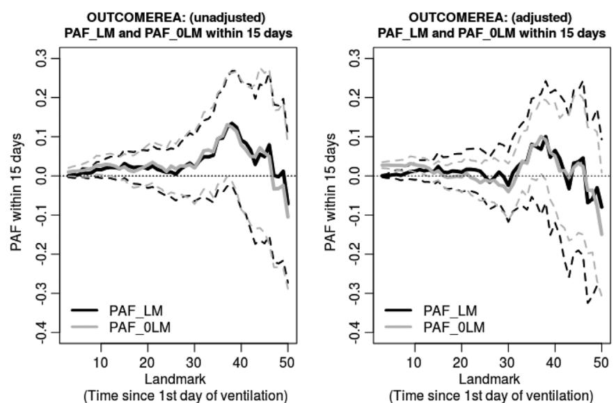
FIGURE 7 Unadjusted estimates of PAF_{LM,h} and PAF_{0LM,h} (left panel) and the adjusted estimates (right panel) of our sample of the OUTCOMEREA database. The dashed lines are the pointwise 95%-CI intervals of the separate models of PAF_{LM,h} (black) and PAF_{0LM,h} (gray)
