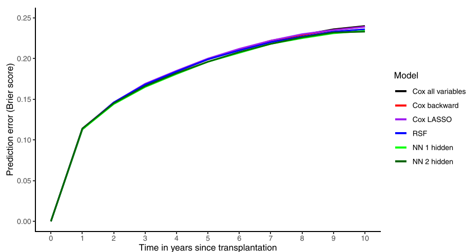
Fig. 1 Prediction error curves for all models
