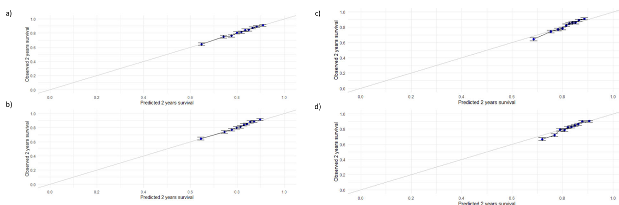
Fig. 3 Calibration plots at 2 years on the test data: a Cox model with all variables, b Random Survival Forest, c Partial Logistic Artificial Neural Network with 1 hidden layer, d Partial Logistic Artificial Neural Network with 2 hidden layers
