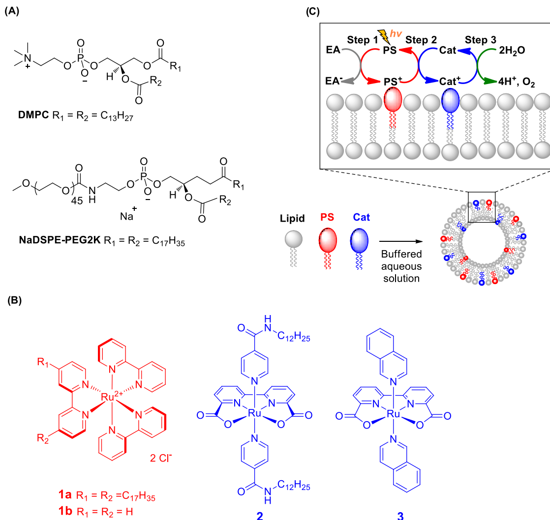
Scheme 1. Chemical Structures of (A) Phospholipids (DMPC) 1,2-Dimyristoyl- sn -glycero-3-phosphocholine and (NaDSPE-PEG2K) 1,2-Distearoyl- sn -glycero-3-phosphoethanolamine- N -[methoxy(polyethyleneglycol)-2000] Sodium Salt, and (B) Lipophilic (1a, 2) and Water-Soluble (1b, 3) Water Oxidation Catalysts and Alkyl-Functionalized Ruthenium Tris-Bipyridine Photosensitizer Utilized in This Study. (C) Schematic of a Molecularly Functionalized Liposome System, with the Inset Highlighting a Simplified Representation of Different Electron Transfer (ET) Steps Occurring during Photocatalytic Water Oxidation on the Water–Membrane Interfaces a
