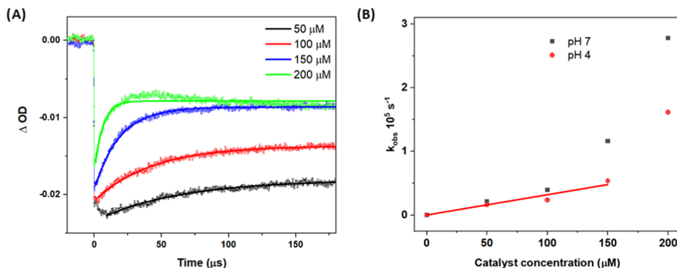
Figure 5. (A) Transient absorption traces at 450 nm after laser flash excitation of homogeneous, aqueous solutions containing 20 \mu M 1b , 5 mM Na_2S_2O_8 , 50 mM phosphate buffer (pH = 4) and different concentrations of catalyst 3 (50, 100, 150, or 200 \mu M ). The figure also includes monoexponential fits yielding k_{obs} . Excitation with 8 ns 460 nm pulsed light. (B) Observed pseudo-first-order rate constants ( k_{obs} ) for electron transfer from 3 to PS vs concentration of 3 , at pH = 4 and 7. A linear fit to the data at pH = 4 with [3] = 0 –150 \mu M gave a hole transfer rate constant k = 3.2 \times 10^8 M^{-1} s^{-1} .
