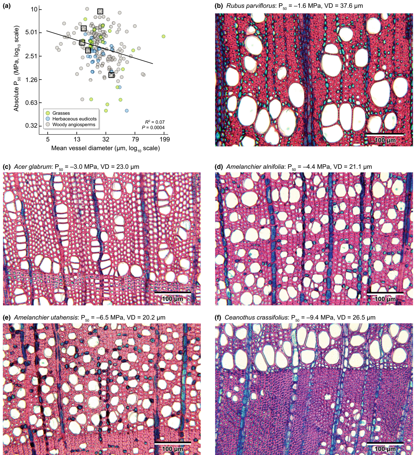
Fig. 1 Weak correlation between the xylem pressure inducing 50% loss of hydraulic conductivity ( P_{50} ) and mean vessel diameter (VD) across angiosperm branches from 186 species belonging to 51 families based on linear regression analysis (a), illustrated with light microscope images from transverse sections (b–f) of species represented by rectangles in (a). Species with narrow vessels ( < 20 \mu\text{m} ) have a higher chance to be embolism resistant, but there is large scatter in P_{50} for a given vessel diameter. Microscopic illustrations are taken from samples of the same individuals/populations measured for embolism resistance. P_{50} and vessel diameter (based on equivalent circle diameter) are taken from the revised dataset of Lens et al. (2016), which is based on the original dataset of Choat et al. (2012) with exponential vulnerability curves removed (see Fig. S1 for a graph with exponential vulnerability curves included). Dataset is included in Table S1.
