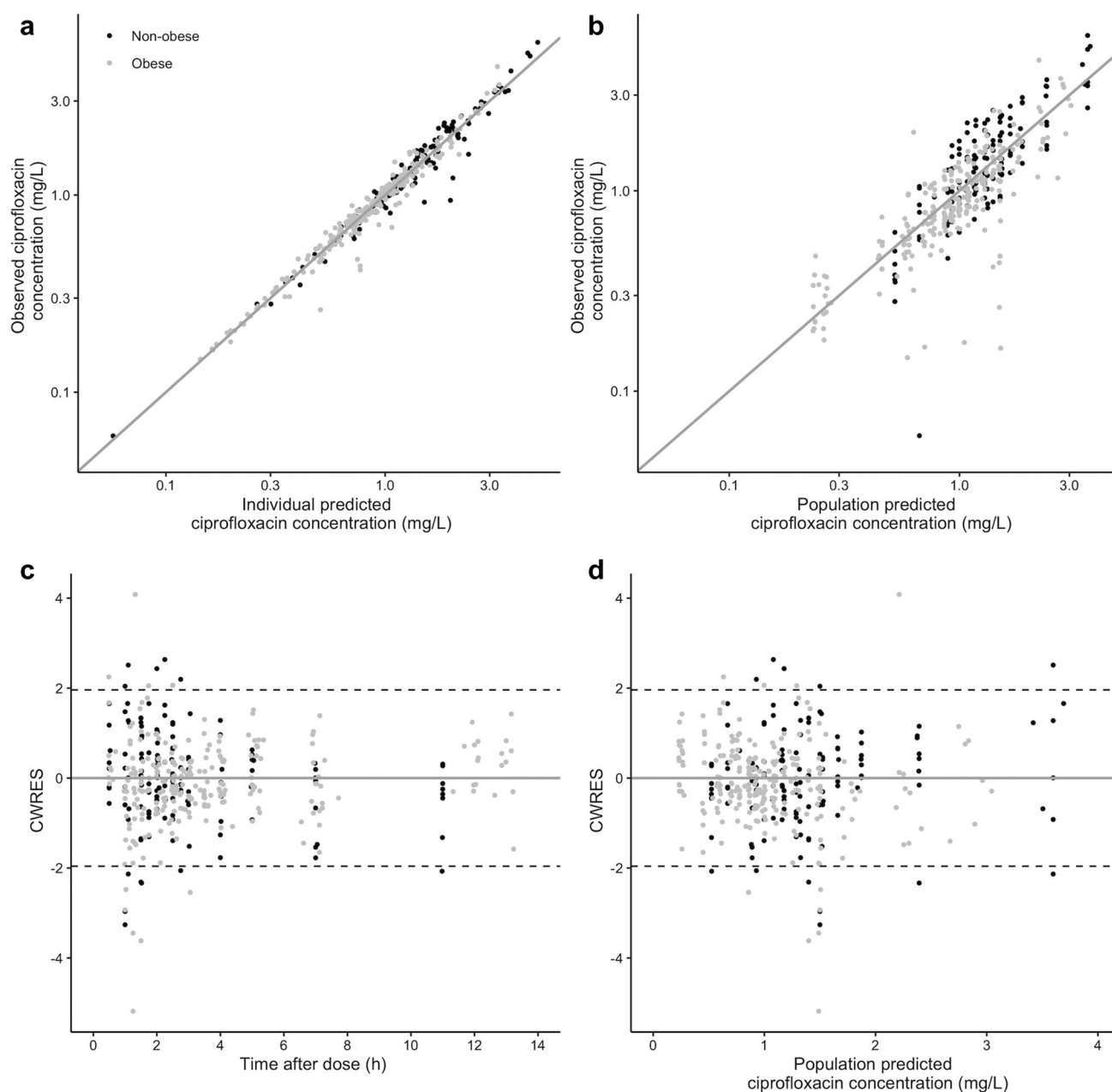
Fig. 1 Diagnostic plots of the final model for morbidly obese individuals (grey dots) and non-obese individuals (black dots). a Observed versus individual predicted ciprofloxacin concentrations. b Observed versus population predicted ciprofloxacin concentrations. c CWRES versus time after dose. d Conditional weighted residuals versus pop-
