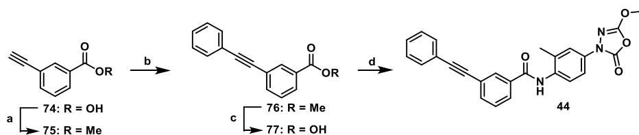
Scheme S3.4 | Synthesis of compound 44 . Reagents and conditions: a) MeI, K 2 CO 3 , DMF, 0°C to RT, 96%; b) iodobenzene, CuI, PPh 3 , Pd(PPh 3 ) 2 Cl 2 , Et 3 N, 40°C, 75%; c) KOH, MeOH/THF, RT, 72%; d) 6 , PyAOP, DIPEA, ACN, RT, 71%.
