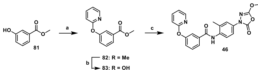
Scheme S3.7 | Synthesis of compound 46 . Reagents and conditions: a) 2-bromopyridine, picolinic acid, K 3 PO 4 , CuI, DMSO, 110°C, 28%; b) 6M HCl (aq.), 110°C, 89%.
