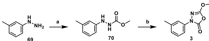
Scheme S3.2 | Synthesis of compound 3 . Reagents and conditions: a) methyl chloroformate, pyridine, DCM, 0°C to RT, 60%; b) \text{COCl}_2 , pyridine, DCM, 0°C, 58%.
