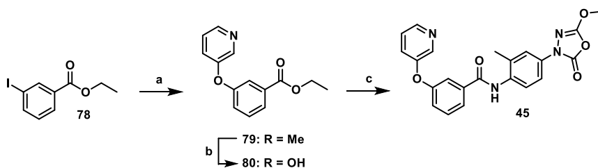
Scheme S3.6 | Synthesis of compound 45 . Reagents and conditions: a) pyridin-3-ol, picolinic acid, K 3 PO 4 , CuI, DMSO, 110°C, 36%; b) 6M HCl (aq.), 110°C, 89%.
