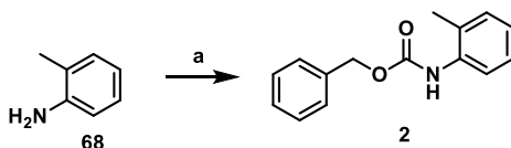
Scheme S3.1 | Synthesis of compound 2 . Reagents and conditions: a) benzyl chloroformate, pyridine, DCM, 0°C to RT, quant.
