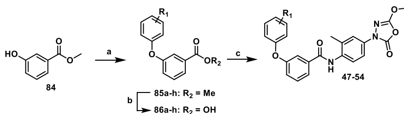
Scheme S3.5 | Synthesis of building blocks 86a-h . Reagents and conditions: a) RB(OH) 2 , Cu(OAc) 2 , Et 3 N, air, DCM, RT, 25% – 34%; b) KOH, MeOH, RT or 55°C, 83 – 94%.
