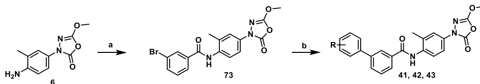
Scheme S3.3 | Synthesis of compounds 41-43 . Reagents and conditions: a) 2-bromobenzoic acid, PyAOP, DIPEA, ACN, RT, 43%; b) \text{RPhB(OH)}_2 , \text{K}_2\text{CO}_3 , \text{Pd(PPh}_3)_4 , \text{H}_2\text{O/dioxane} , 45°C, 26% – 64%.
