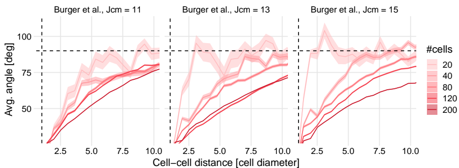
Figure S5.9: Influence of surface energy J_{cell,med} and of cell density on stream formation. Results are shown for the proposed persistence model with strong pseudopod coordination.
