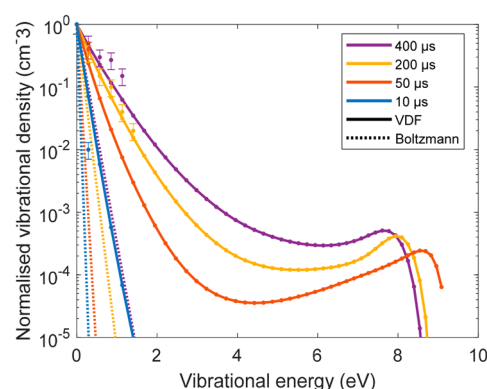
Figure 15. Calculated VDFs (solid lines) and measured VDFs (data points) in the last pulse of the plasma, for four different pulse widths and a pulse frequency of 1 kHz. In addition, the Boltzmann distribution functions at the corresponding gas temperatures (cf. Figure 11) are plotted in dashed lines, to indicate the strong degree of vibrational nonequilibrium.
