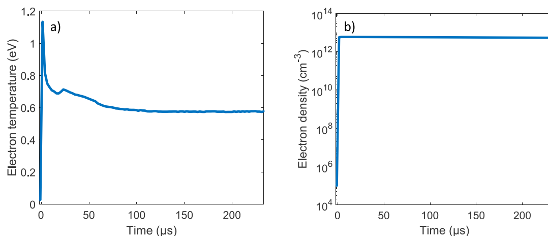
Figure 5. Time evolution of (a) the calculated electron temperature and (b) the calculated electron density through the 233 \mu s pulse.
