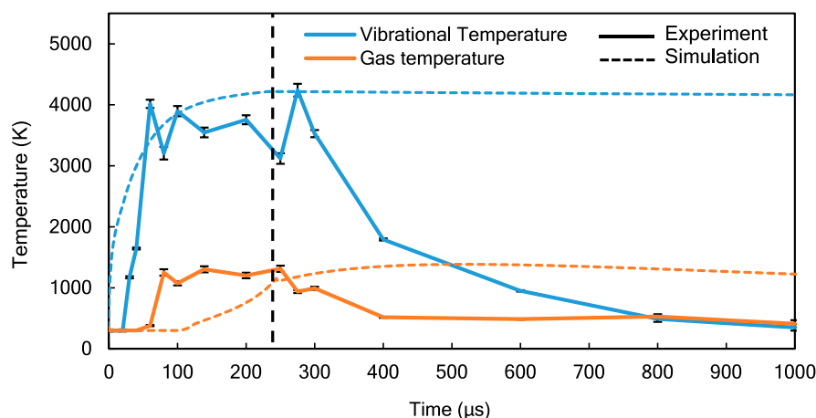
Figure 3. Time-evolution of the measured (full lines) and calculated (dashed lines) vibrational and gas temperature through a 233 \mu s pulse. The error bars of the experimental values are the errors resulting from the fitting procedure. The measured values are obtained in the center of the plasma. The end of the pulse is indicated with a vertical dashed line.
