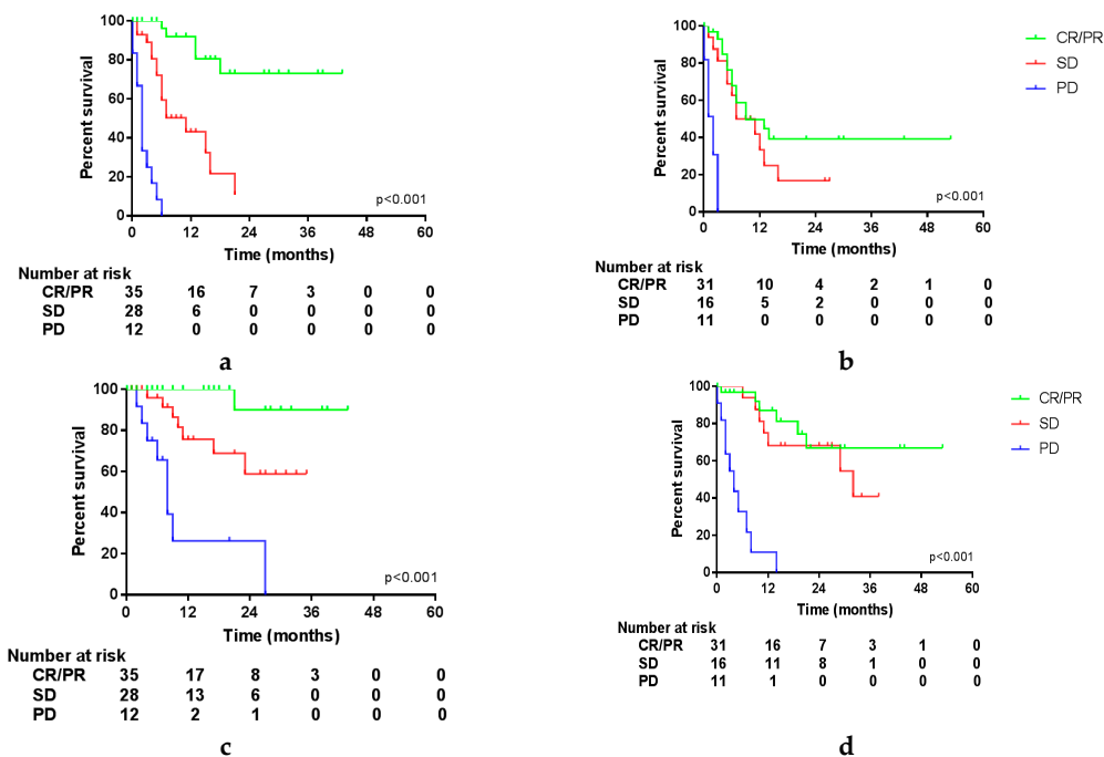
Figure 2. Survival per status of disease at first follow-up after surgery. (a) Progression-free survival (PFS) in patients treated with ICI; (b) PFS in patients treated with targeted therapy; (c) overall survival (OS) in patients treated with ICI; (d) OS in patients treated with targeted therapy.
