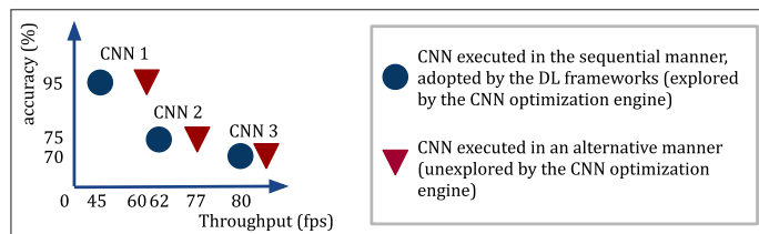
Figure 1.4: CNNs associated with alternative manners of execution
