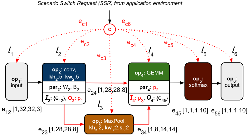
Figure 5.4: SBRs MoC
