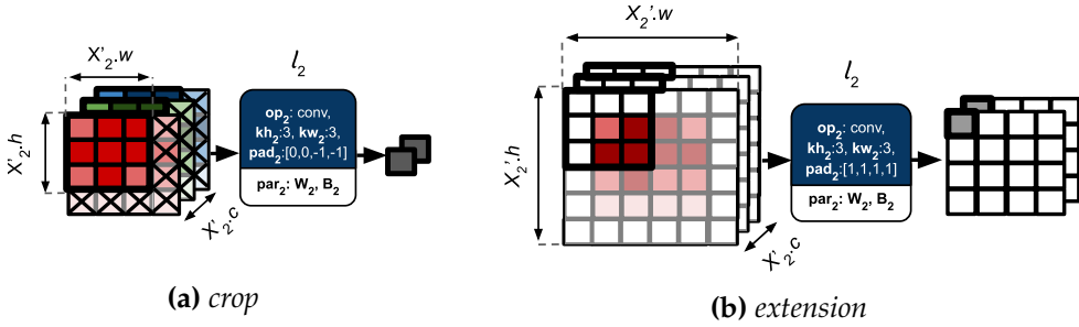
Figure 2.3: Padding
