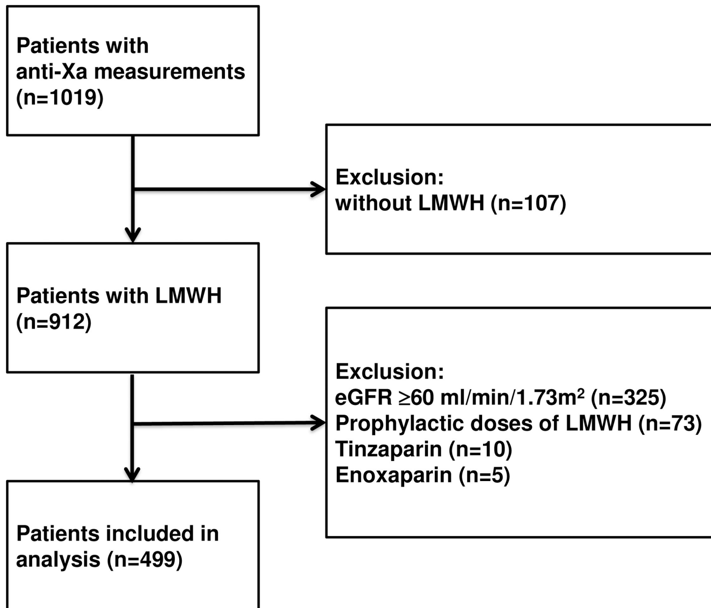
Fig 1. Study outline.
