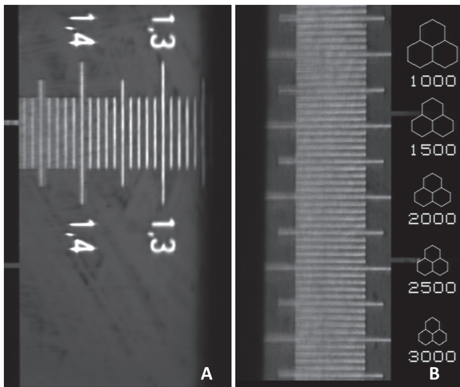
Figure 2. Picture of the micro-ruler used for external calibration, photographed with our specular microscopes.
