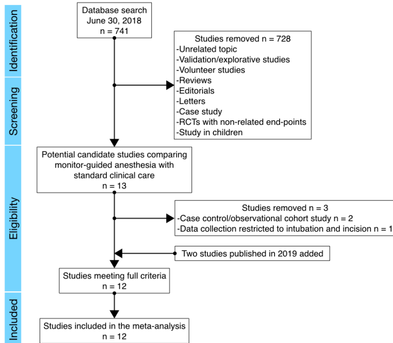
Figure 1. Flow diagram of the study selection process following the PubMed search on June 30, 2018.
