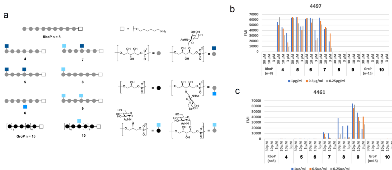
Figure 3. (a) Schematic overview of the TA microarray library. Microarray results for (b) mAb 4497 and (c) mAb 4461 at different concentrations. Legend: 1 μg/mL, blue; 0.5 μg/mL, orange; 0.25 μg/mL, gray. Values refer to the average of the fluorescent median intensity of three spots for each compound printed at 30, 10, and 3 μM concentrations. n = number of repeating units.
