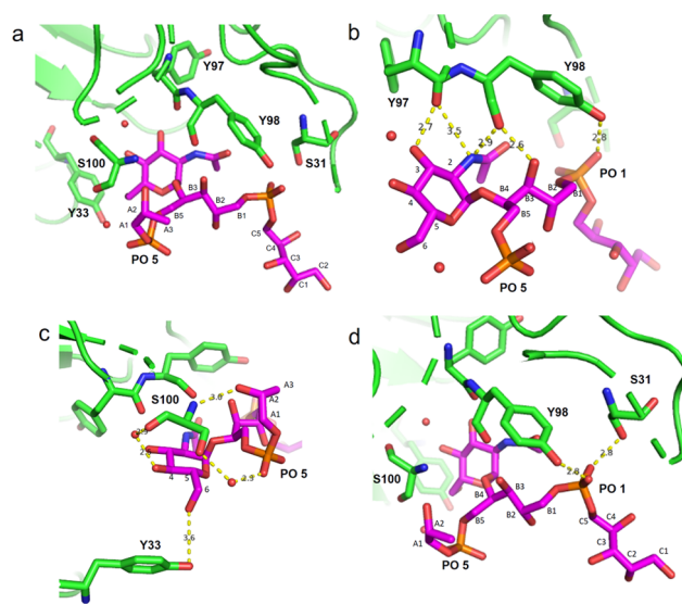
Figure 4. Different views of the binding site of IgG mAb 4461 in complex with (α-1,4)-GlcNAc WTA (ligand 1). (a) The α-GlcNAc-modified WTA 1 is bound in a cavity formed between the CDR of the heavy and light chains of the antibody. Residues S31, Y97, Y98, S100, and Y33 are involved in H-bond interactions with the ligand. (b) Residues Y97 and Y98 establish H-bonds with the GlcNAc ring, with the phosphate group 1, and with the Rbo-B3 OH. (c) Residue S100 forms a H-bond with the Rbo-A2 OH as well as the GlcNAc C4-OH and phosphate group 5 through a water molecule. Residue Y33 interacts via an H-bond with GlcNAc C6-OH. (d) Residues S31 and Y98 establish H-bonds with an oxygen atom of phosphate group 1. The ligand (α-1,4)-GlcNAc WTA 1 is shown in magenta.
