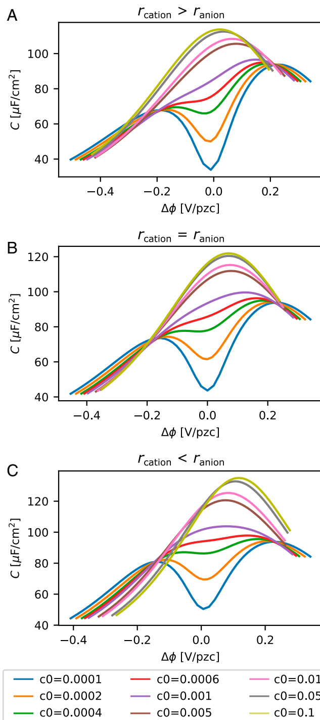
Fig. 10. Model results: water adsorption + ion attraction. (A) The cation has a larger hydrated ion radius than the anion (model for \text{LiClO}_4 ; x_{rep}^{\text{cat}} \approx 4 Å, x_{rep}^{\text{an}} \approx 3 Å). (B) The cation and anion have the same hydrated ion size (model for \text{NaClO}_4 ; x_{rep}^{\text{cat}} \approx 3 Å, x_{rep}^{\text{an}} \approx 3 Å) and (C) the cation has a smaller hydrated ion radius than the anion (model for \text{CsClO}_4 ; x_{rep}^{\text{cat}} \approx 4 Å, x_{rep}^{\text{an}} \approx 3 Å). All other parameters are identical to Fig. 9A.
