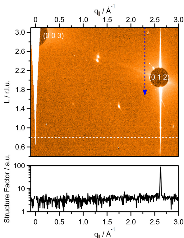
Fig. 8. Ordered oxide: the maximum intensity from a series of detector images from a (0 1) CTR measurement after applying 1.35 V for 60 min. The blue dashed line indicates the q_{\parallel} value where a signal due to the formation of 7/8-strips would appear. The white dashed line indicates the L-value which was used to extract the profile shown in the bottom panel. (For interpretation of the references to colour in this figure legend, the reader is referred to the web version of this article.)
