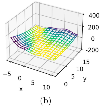
Branin low-fidelity: A=0.90
