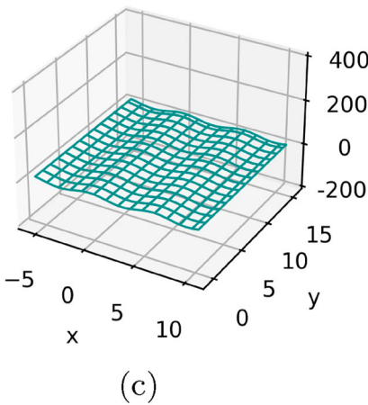
Figure 4. Adjustable multi-fidelity function example showing the adjustable Branin function: (a) high-fidelity; (b), (c) and (d) low-fidelity for A = 0.1, 0.5 and 0.9 , respectively. 9,10
