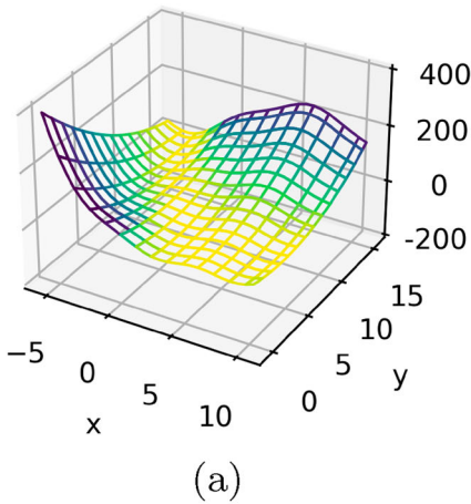
Branin low-fidelity: A=0.50
