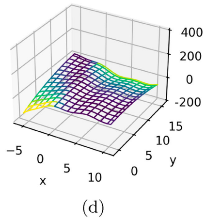
Figure 4. Adjustable multi-fidelity function example showing the adjustable Branin function: (a) high-fidelity; (b), (c) and (d) low-fidelity for A = 0.1, 0.5 and 0.9 , respectively. 9,10
