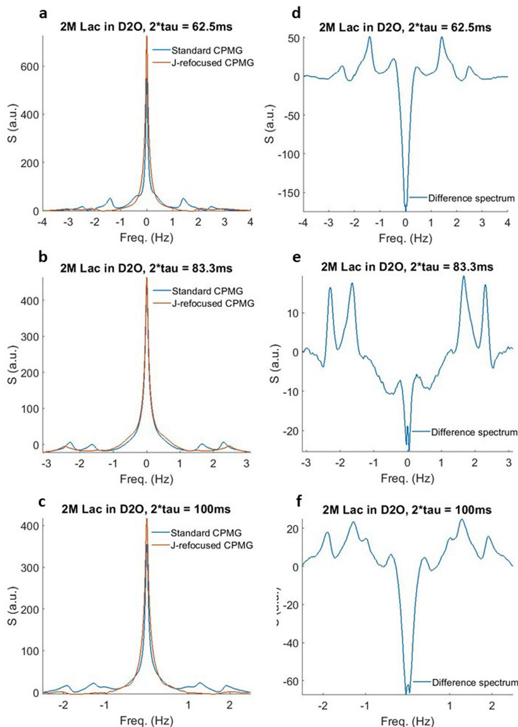
Fig. 6. (a–c) J-spectra of 2 M lactate in D 2 O acquired with the standard CPMG sequence (blue) and the J-refocused CPMG sequence (brown). The decoupling effect of the J-refocused CPMG sequence is incomplete (see for example the peaks at \pm 2.5 Hz in (b)), but the majority of the J-modulation is suppressed. (d–f) Difference spectra obtained by subtracting the J-refocused spectra from the standard ones. In all spectra the bandwidth is 1/(4\tau) and not 1/(2\tau) , as data in the J-refocused CPMG are acquired every other echo. (For interpretation of the references to colour in this figure legend, the reader is referred to the web version of this article.)
