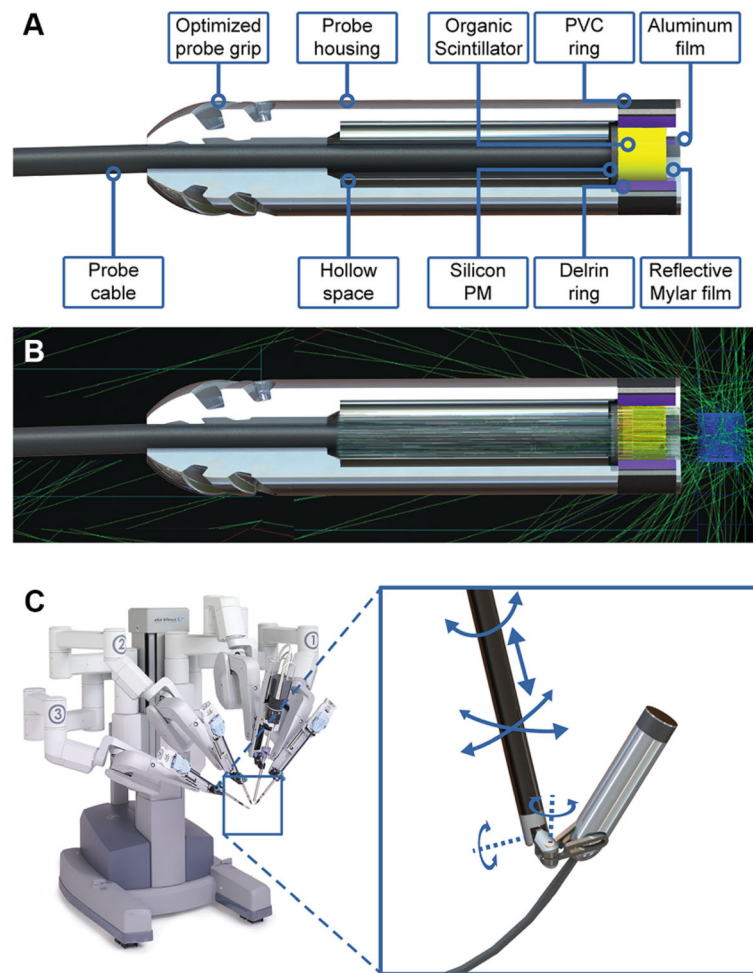
Fig. 1 DROP-IN \beta probe design. a Schematic representation of the probe components. b Example of one of the Monte Carlo simulations optimizing \beta -particle detection and \gamma -photon transparency. c Overview of the probe application setup, showing its high maneuverability
