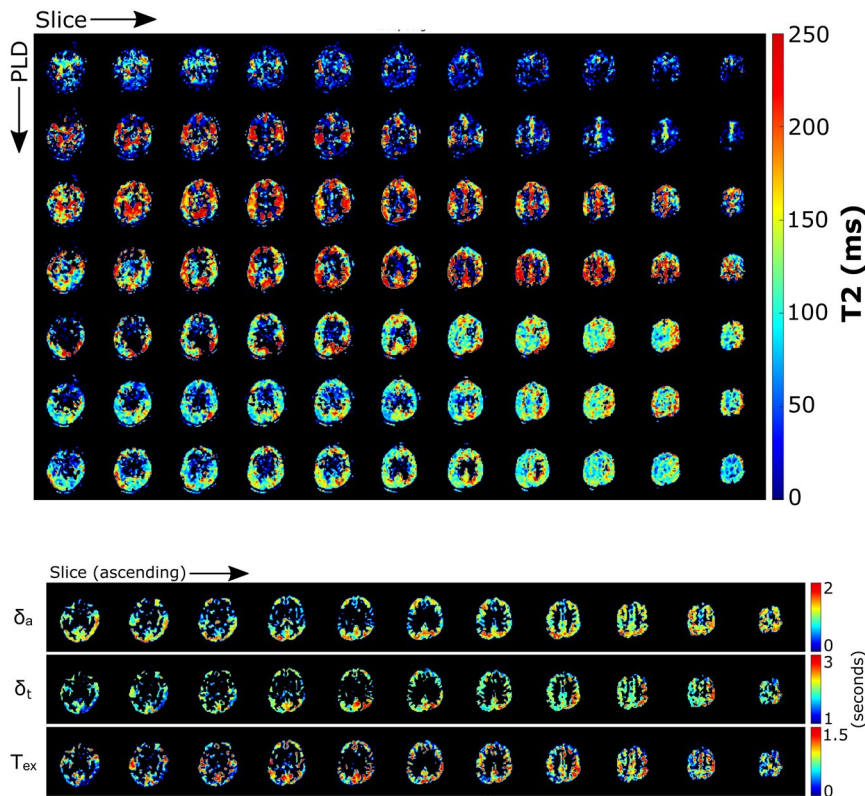
FIGURE 7 Map of the T_2 calculated on the 3D-acquired data set with the TRUST technique, for all time points. Voxels with an uncertainty on the fit higher than 200 ms or lower than 0.5 ms were removed from this image (ill-fitting points)
