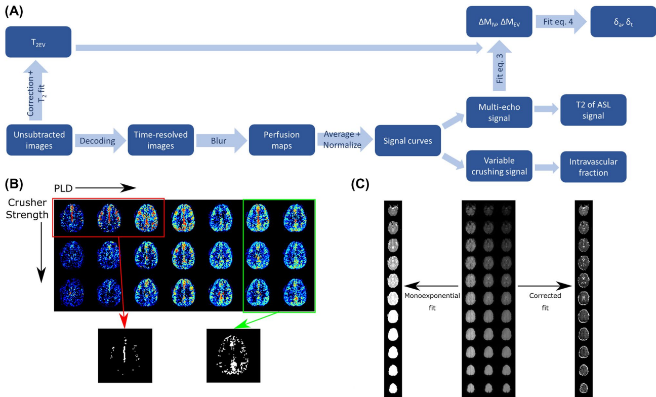
FIGURE 2 A, Data analysis pipeline. B, The masking step. The three earliest time points of the uncrushed perfusion maps are averaged and thresholded to obtain the vascular mask. The two last time points of images from all crusher settings are averaged and thresholded for the gray-matter mask, and any voxels from the arterial mask are removed. C, The T_{2EV} maps without (left) and with (right) correction for the sequential slice acquisition
