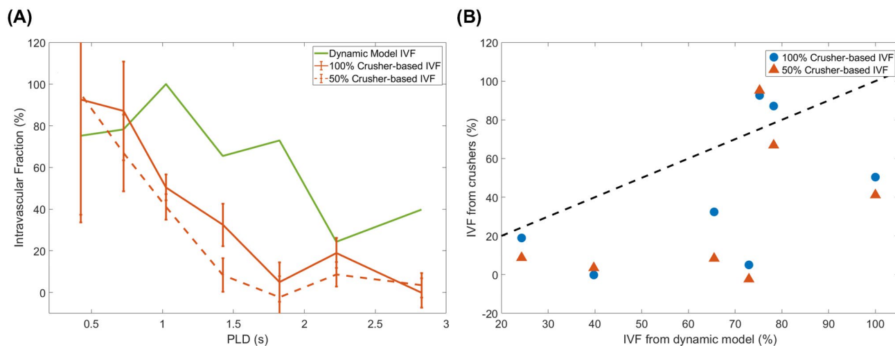
FIGURE 6 Comparison of the intravascular fractions (IVFs) as calculated with both methods. A, The IVFs are shown through time, for the crusher-gradient technique (orange) and the compartmental model applied to the variable eTE data (green). B, Scatterplot showing the direct comparison of IVF values from both techniques (the black dotted line represents a perfect match)
