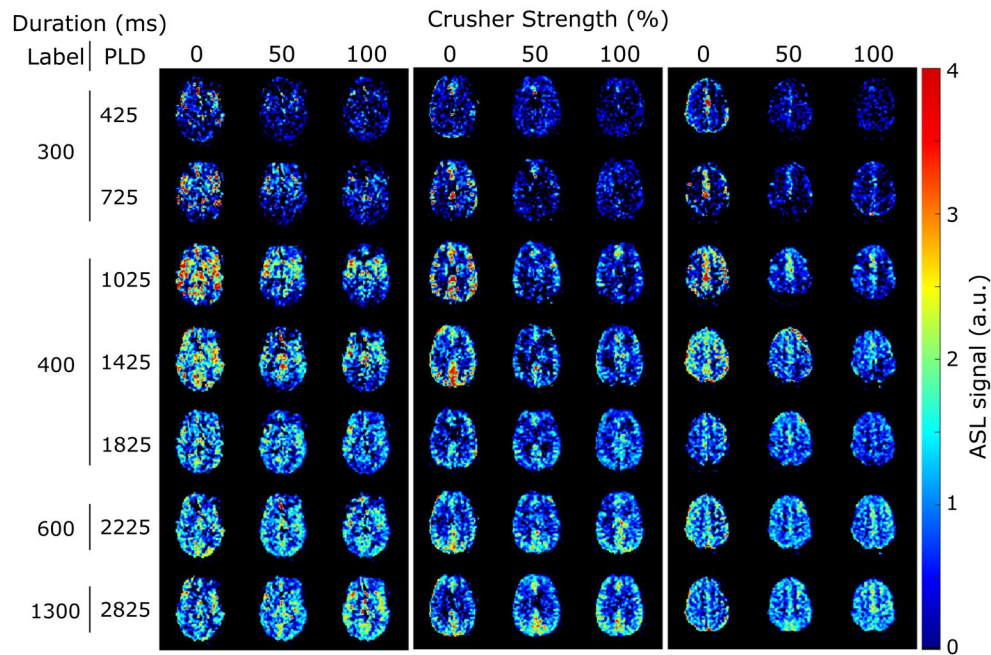
FIGURE 3 Arterial spin labeling (ASL) signal maps with variable crushing at all time points in three slices of 1 subject. All images were acquired with an eTE of 0 ms
