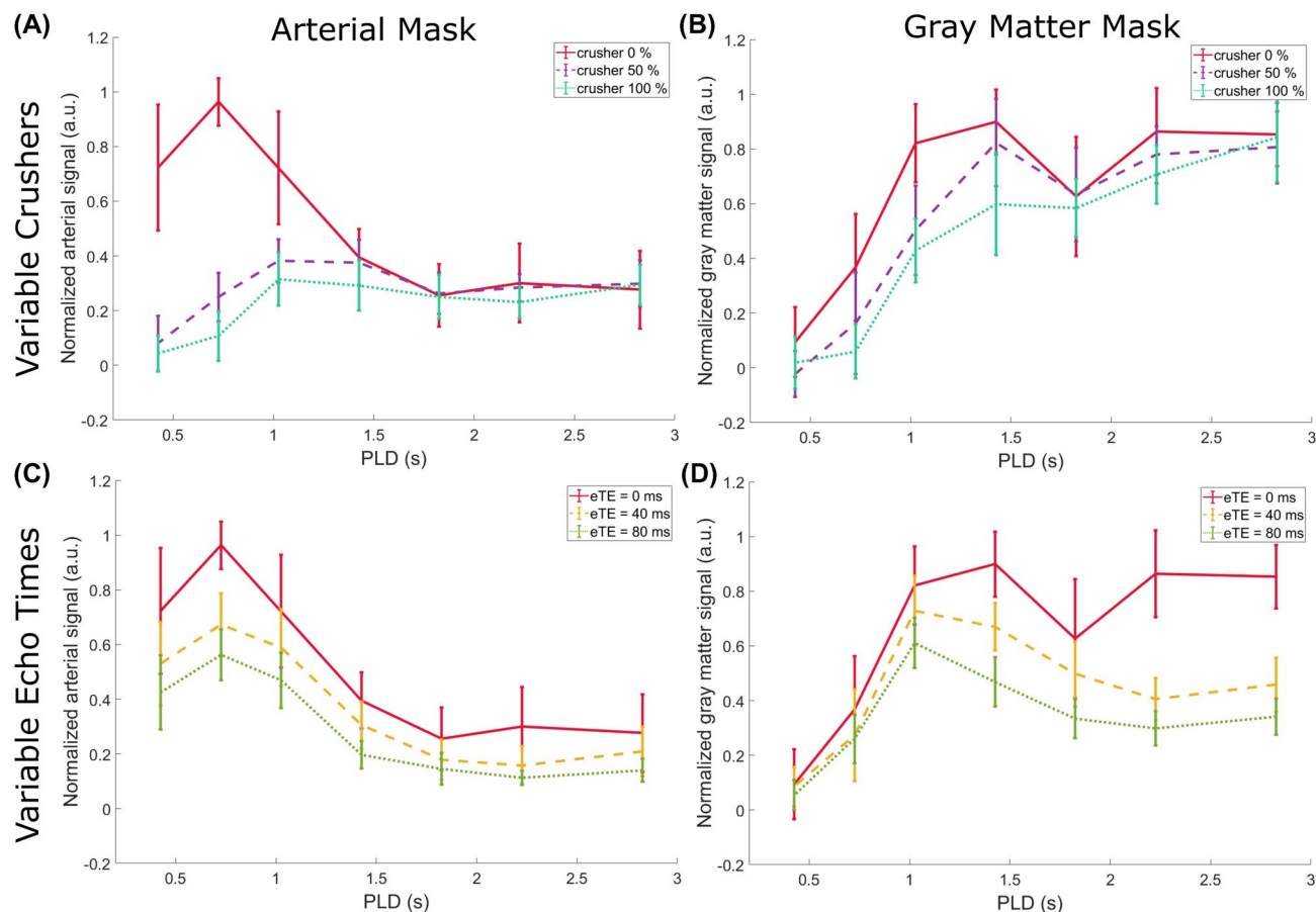
FIGURE 4 Average normalized gray matter and arterial signal through time, showing effects of crushers and TEs. Error bars indicate the SEM of the subjects
