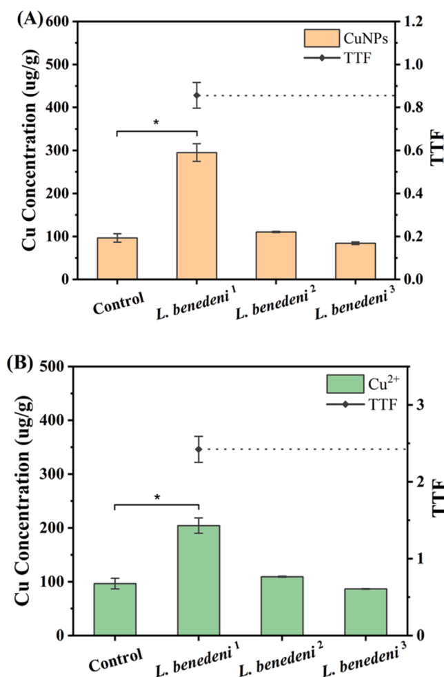
Fig. 3. Cu concentrations ( \mu\text{g/g} dry weight) for CuNPs (A) and Cu 2+ (B) in mysids ( L. benedeni ) and their mass-based trophic transfer factors (TTF). L. benedeni 1 , L. benedeni 2 and L. benedeni 3 stand for the predators in case-1 (from alga to mysid), case-2 (from daphnia to mysid), and case-3 (from alga through daphnia to mysid). Control stands for the mysid fed by unexposed food. Bars represent mean \pm standard deviation ( n = 3 ). The asterisk indicates statistical significance versus control group ( p < 0.05 ).
