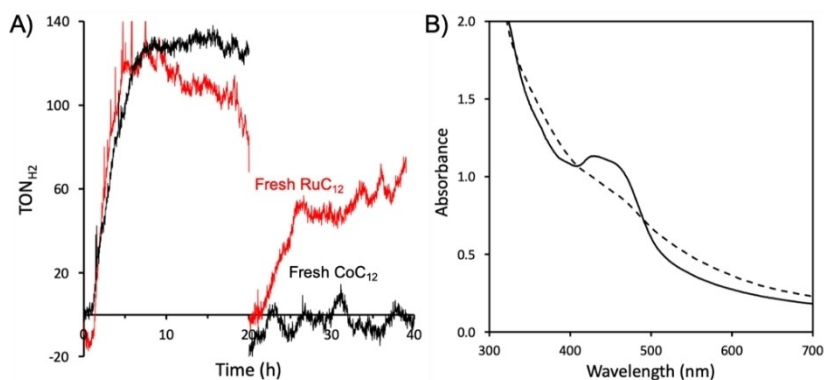
Figure 5. (A) Repetitive photocatalytic proton reduction using a liposome mixture consisting of 5 mM DPPC, 50 \mu M NaDSPE-PEG2K, 50 \mu M \text{RuC}_{12} , 5 \mu M \text{CoC}_{12} in argon-saturated 0.1 M NaHAsc and 0.1 M TCEP aqueous solution (3.5 mL, pH = 4.0) at 25 ^{\circ}\text{C} . The samples were left in the dark for 1 h and afterwards irradiated with blue light ( \lambda_{\text{irr}} = 450 nm, P = 10.6 mW, \Phi_0 = 13.7 nmol/s) for 19 h. Afterwards, additional 50 \mu M \text{RuC}_{12} (red curve) or 5 \mu M \text{CoC}_{12} (black curve) was added to the reaction mixture and photocatalysis was started again. Bulk concentrations [\text{RuC}_{12}] and [\text{CoC}_{12}] indicate theoretical concentrations assuming no losses during liposome preparation. (B) UV-Vis spectrum of the reaction solution before irradiation (solid line) and after irradiation (dashed line).
