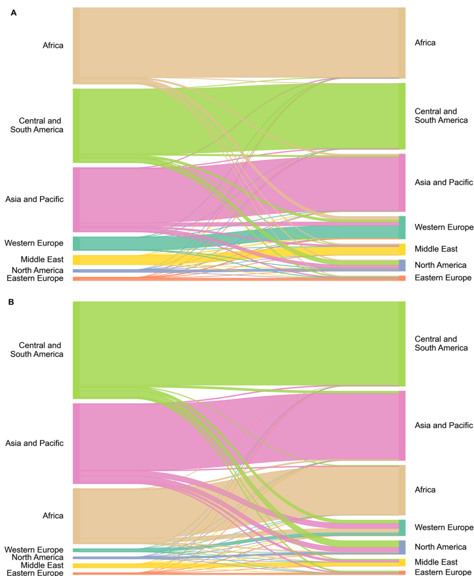
Figure 3. Embodied biodiversity loss flows for (A) plants and (B) vertebrates (mammals, birds, amphibians, and reptiles) from land use within KBAs. Producing regions are on the left of the figure, consuming regions on the right. Regions are ordered by the magnitude of loss in the consuming region. The width of the flows is proportional to the magnitude of the potential global species loss.
