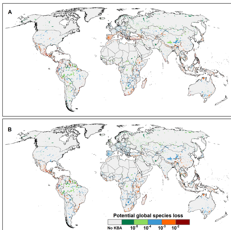
Figure 1. Potential global species loss driven by land use within KBAs for (A) plants and (B) vertebrates (mammals, birds, amphibians, and reptiles). The results are the sum of potential global species loss across all land-use types and intensities driven by consumption of countries.
