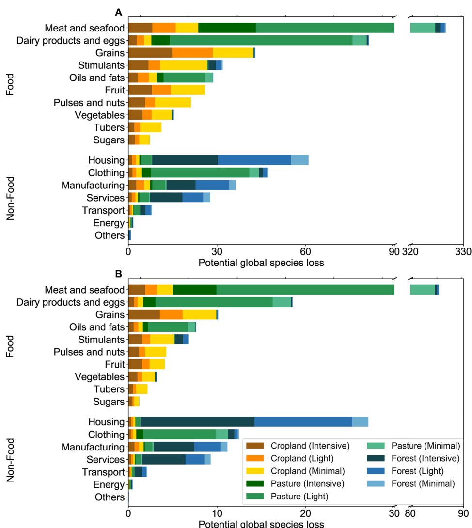
Figure 4. Potential global species loss due to specific product consumption from land use within KBAs for (A) plants and (B) vertebrates (mammals, birds, amphibians, and reptiles). Forest includes managed and planted forests.
