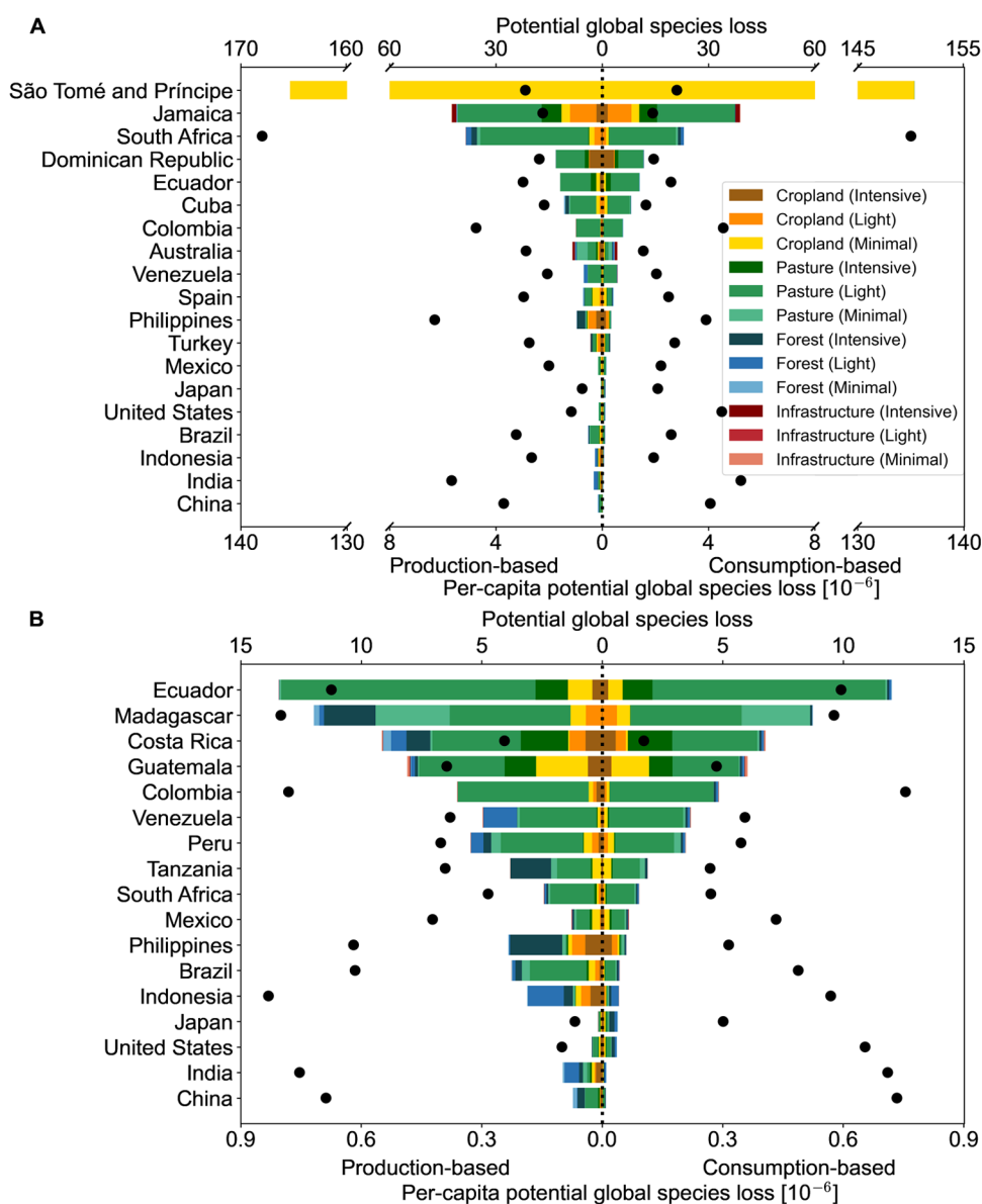
Figure 2. Potential global species loss from land use within KBAs for (A) plants and (B) vertebrates (mammals, birds, amphibians, and reptiles). On the x -axis, the production-based perspective is shown to the left of zero and the consumption-based perspective to the right. The y -axis lists the top 15 countries/regions with the largest consumption-based or production-based biodiversity loss from land use within KBAs at the national level. Since there are some differences in the top 15 from the two perspectives, the overall number is larger than 15. The bars show the per-capita values of biodiversity loss within KBAs per land-use type and intensity. The points show the total national biodiversity loss with a value shown by the upper x -axes on top of each plot. Forest includes managed and planted forests.
