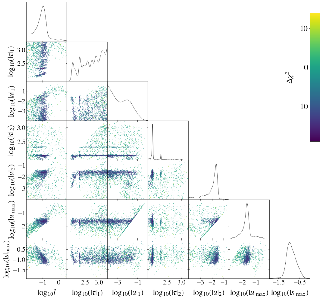
Figure 2.6: Posterior distribution for the reconstruction of the speed of sound’s profile u(\tau) using 2 training nodes and the logarithmic parametrization shown in Figure 2.2. We use \Delta\chi^2 = \chi_{\text{model}}^2 - \chi_{\text{baseline}}^2 as the variable for the scatter plot’s colour scale, the reference \chi_{\text{baseline}}^2 corresponding to the MAP of the baseline \Lambda\text{CDM} model to the same datasets. We show the parameters of the training nodes ( \tau_i, u_i ) and the correlation length l (described in 2.3.1; priors in 2.3.2). We also show the posteriors of the EFT parameters ( |u|_{\text{max}}, |s|_{\text{max}} ) (described in section 2.2, and not sampled directly, but derived from the nodes parameters). It can be seen how longer correlation lengths (broader reductions) lead to lower values of |s|_{\text{max}} , and vice-versa. The posterior distributions for different numbers of nodes display similar patterns. For all cases, the posterior distributions are clearly multi-modal.
