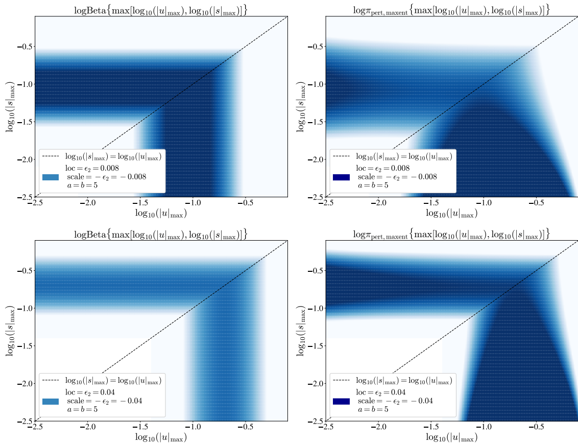
Figure 2.3: A description of the Bayesian priors adopted in this study. Left panels: Desired Beta density distribution for the parameters \log_{10}(|u|_{\max}) and \log_{10}(|s|_{\max}) , with \epsilon_2 = 0.008 and \epsilon_2 = 0.04 , respectively. Right panels: probability density distribution induced by \pi_0 on \log_{10}(|s|_{\max}) and \log_{10}(|u|_{\max}) (defined as P in the denominator of equation (2.12)), for a Gaussian-Processes reconstruction in \log|u(\log|\tau)| using 2 training nodes. The initial prior \pi_0(\tau_i, u_i, l) induces overdensities at low \log_{10}(|s|_{\max}) due to this quantity being doubly-correlated to early-time position of the nodes and large correlation lengths; equation (2.12) corrects for this effect.
