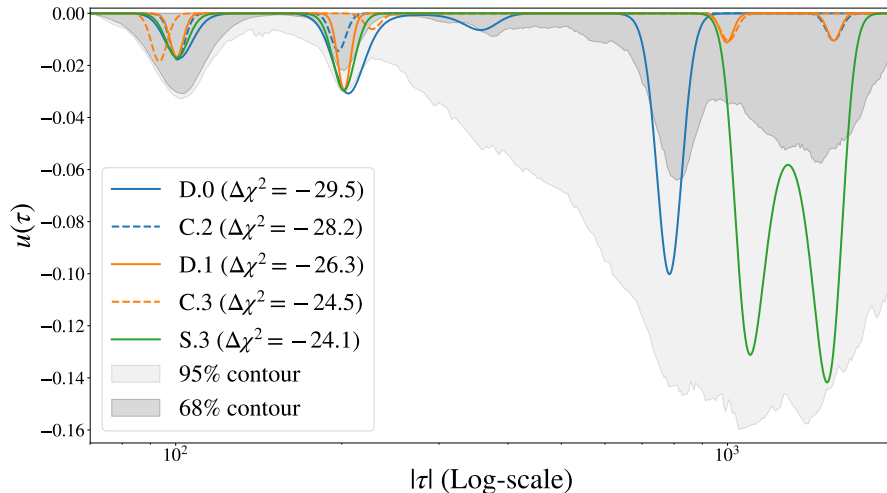
Figure 2.7: Reconstruction of the inflaton’s speed of sound profile u(\tau) based on a 4-nodes GP, where the confidence contours (68% and 95%) are shown. We are able to constrain the shape of the inflaton’s speed of sound more stringently at late times (up to \sim -200 ), whereas the confidence intervals get larger at earlier times (i.e. starting from -800 ). This difference in the constraining power between early and late conformal times is mostly due to early-time reductions being associated to low-multipole features where cosmic variance is largest. The best maxima a posteriori are also plotted on top of the confidence contours: two 3-dipped cases (labelled C.2, dashed blue, and C.3, dashed orange), two 4-dipped cases (labelled D.0, solid blue, and D.1, solid orange) and a 3-dipped case in which one of the dips possesses some substructure (labelled S.3, solid green). For additional fits and a more detailed presentation of them see appendix 2.6.
