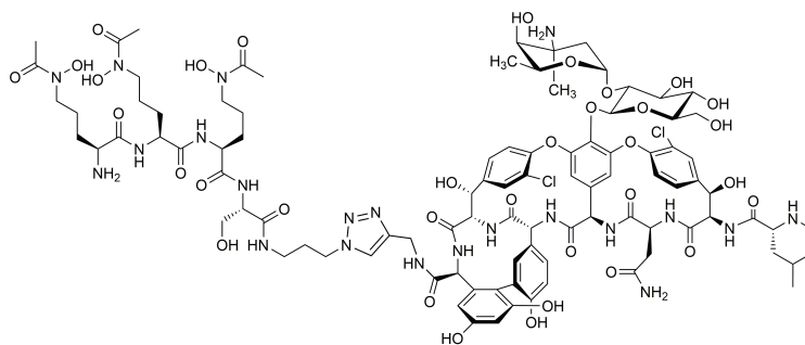
Fig. 7. Representatieve vancomycine-sideromycine
