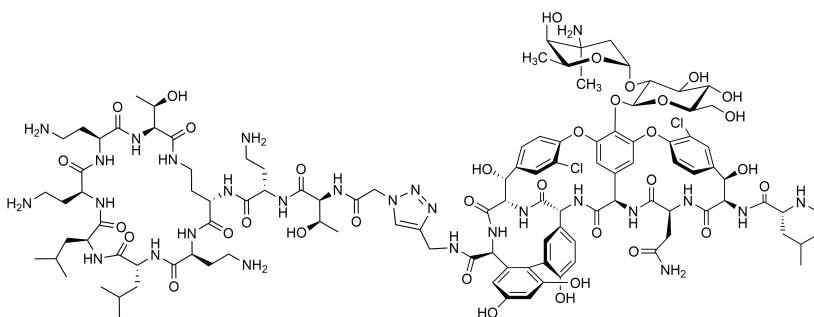
Fig. 6. Representatieve vancomyxin
