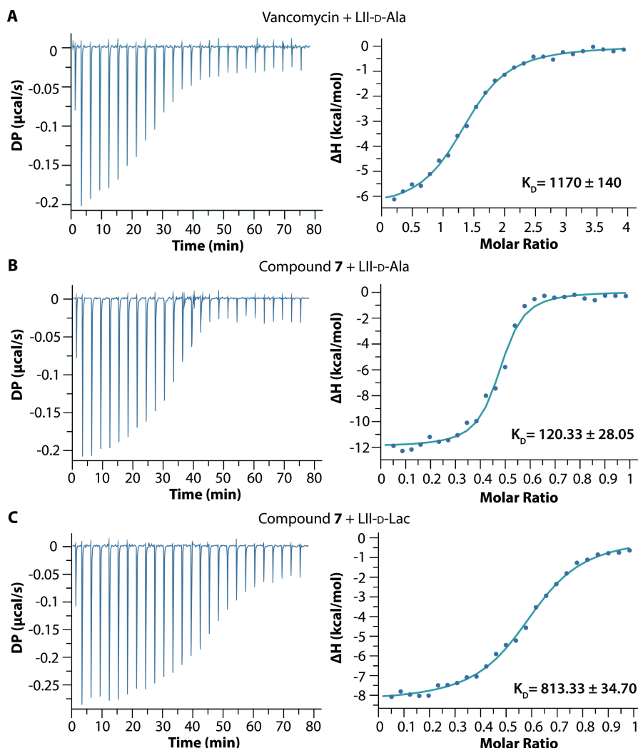
Fig. 6. Lipid II binding of the guanidino lipoglycopeptides assessed by ITC. (A) Representative binding isotherms for the titrations of 200 \mu M LII-D-Ala, 10 mM DOPC LUVs to vancomycin (10 \mu M), (B) 100 \mu M LII-D-Ala, 10 mM DOPC LUVs to compound 7 (20 \mu M), and (C) 200 \mu M LII-D-Lac, 10 mM DOPC LUVs to compound 7 (20 \mu M). Titrations performed in triplicates ( n=3 ). A single titration ( n=1 ) is displayed and is representative for all triplicates. See Table S2 for full thermodynamic parameters and Fig. S7–10 for all triplicate titrations. Experiment performed by Ioli Kotsogianni.
