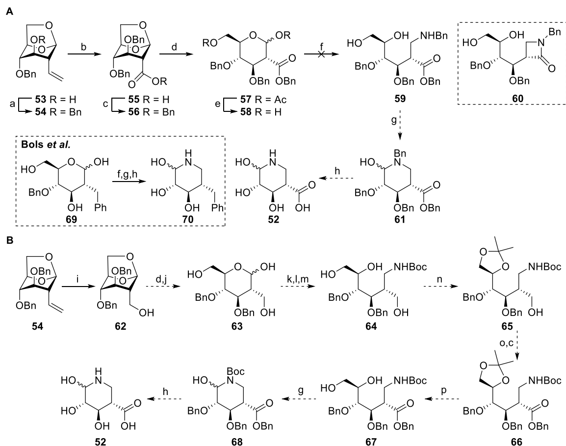
Scheme 6.6. Proposed synthetic schemes for the preparation of glucuronic acid-type noeuromycin 52 . Regents and conditions: a) BnBr, NaH, TBAI, DMF, 0 °C to rt, 79%; b) RuCl 3 ·3H 2 O, NaIO 4 , EtOAc/ACN/H 2 O (2/2/3), rt, 57%; c) BnOH, DIC, DMAP, DCM, 0 °C, 92%; d) TFA, Ac 2 O, 0 °C, 93%; e) p -TsOH, THF/H 2 O (9/1), 70 °C, 82%; f) BnNH 2 , HOAc, NaCNBH 3 , MeOH, 50 °C; g) NaIO 4 , THF/H 2 O, rt; h) Pd/C, H 2 , HCl, EtOH/H 2 O, rt; i) i) OsO 4 , NaIO 4 , dioxane/H 2 O, rt; ii) NaBH 4 , THF/isopropanol, 0 °C, 84% over two steps; j) NaOMe, MeOH; k) allylamine, HOAc, NaCNBH 3 ; l) (Ph 3 P) 3 RhCl, MeCN/H 2 O, reflux; m) Boc 2 O, TEA, DCM; n) p -TsOH, 2,2-dimethoxypropane; o) Jones reagent, acetone; p) 80% HOAc.
