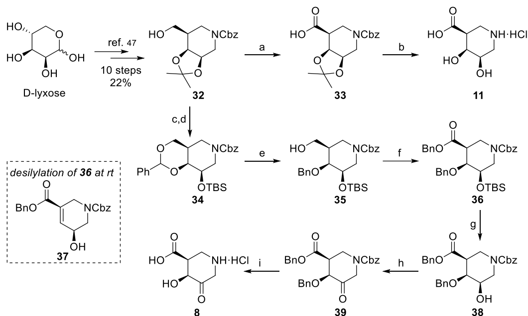
Scheme 5.5. Synthesis of compounds 8 and 11 . Reagents and conditions: a) i ) Dess-Martin periodinane, DCM, rt; ii ) NaClO 2 , NaH 2 PO 4 , 30% H 2 O 2 , CH 3 CN, H 2 O, 0 °C to rt, 65% over two steps; b) H 2 , 10% Pd/C, H 3 O + , THF, rt, quant; c) i ) 8 M HCl, MeOH, rt; ii ) PhCH(OMe) 2 , CSA, DMF, 60 °C; d) TBSCl, imidazole, DCM, rt, 68% over three steps; e) THF·BH 3 , TMSOTf, DCM, 0 °C to rt, 97%; f) i ) Jones reagent, acetone, rt; ii ) benzyl alcohol, DIC, DMAP, DCM, rt, 46% over two steps; g) TBAF (75 wt% in H 2 O), THF, 38 : 0 °C, 5 h, 94%, 37 : rt, overnight, 98%; h) Dess-Martin periodinane, DCM, rt, 71%; i) H 2 , 10% Pd/C, THF, H 3 O + , rt, quant.
