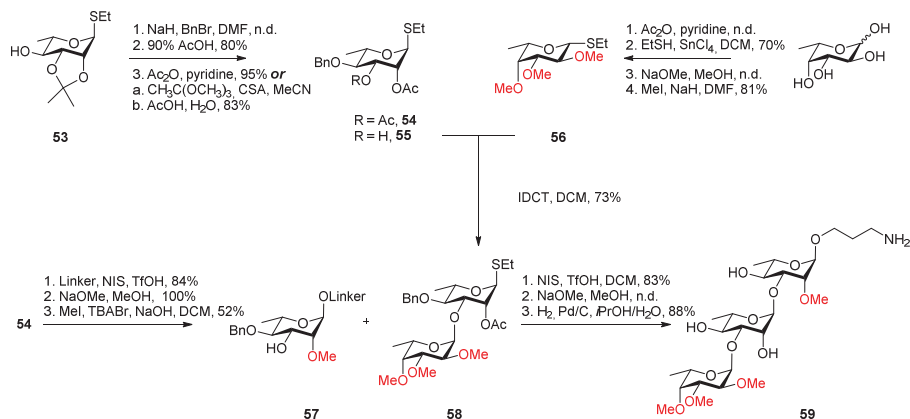
Scheme 9. Synthesis of the PGL-tb1 glycan as reported by van Boom and coworkers in 1990. 76 (n.r. = yield not reported, n.d. = yield not determined)
