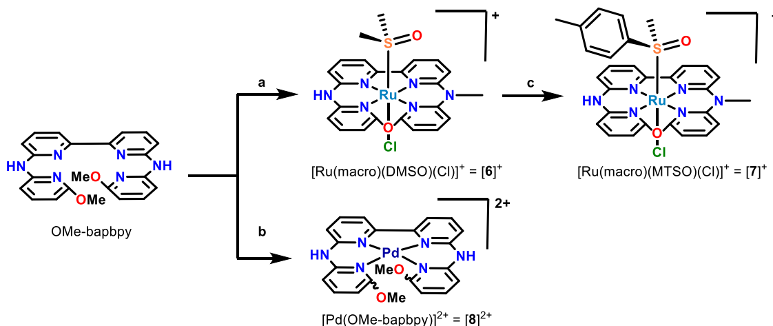
Scheme 1. Synthetic Route Toward Compounds [6]^+ , [7]^+ , and [8]^{2+} a
