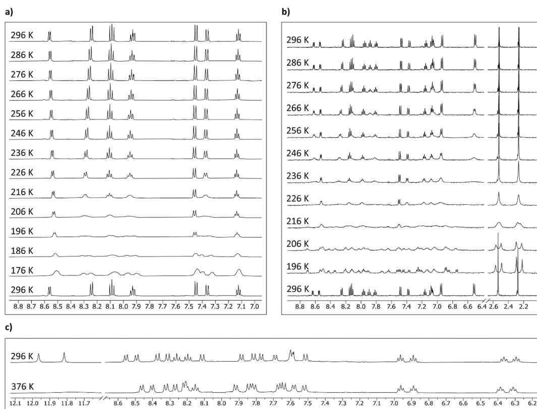
Figure 5. (a) Variable-temperature ^1\text{H} NMR of [1]^+ in methanol- d_4 from 296 to 176 K. (b) [3]^+ in methanol- d_4 from 296 to 196 K. (c) [2]^+ in DMSO- d_6 from 296 to 376 K.
