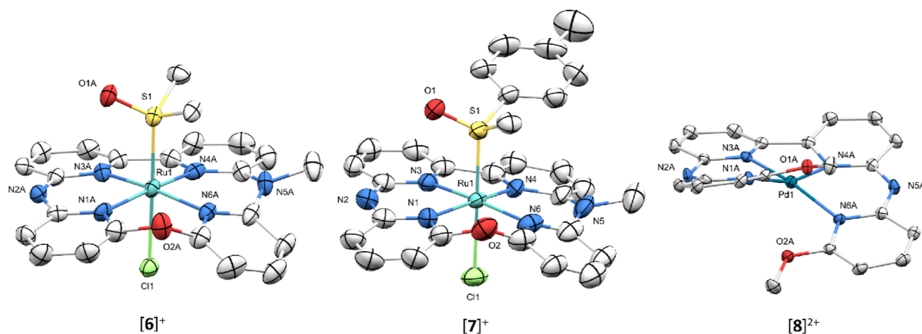
Figure 6. Displacement ellipsoid plots (50% probability level) of the crystal structures of [6]OTf, [7](OTf)·MeOH, and [8](OTf) 2 at 110(2) K. Counterions, hydrogens, and lattice solvent molecules have been omitted for clarity.
