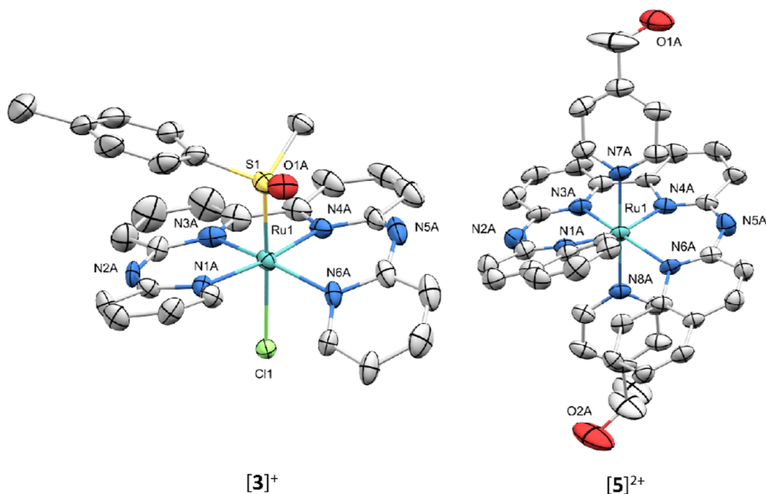
Figure 3. Displacement ellipsoid plots (50% probability level) for [3]\text{PF}_6 and [5](\text{PF}_6)_2 at 110(2) and 173(2) K, respectively. Counterions and hydrogens have been omitted for clarity.
