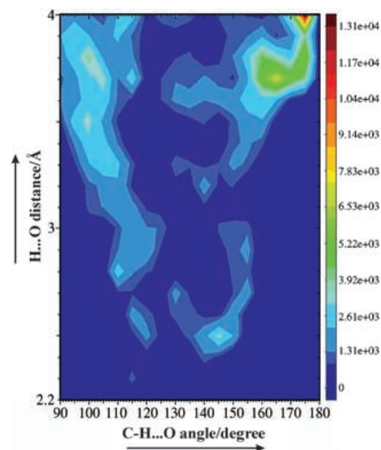
Figure 3. Number of configurations detected along the CPMD simulation with a given H...O distance (H of F_3CH and O of all CO molecules) and C-H...O angle.
