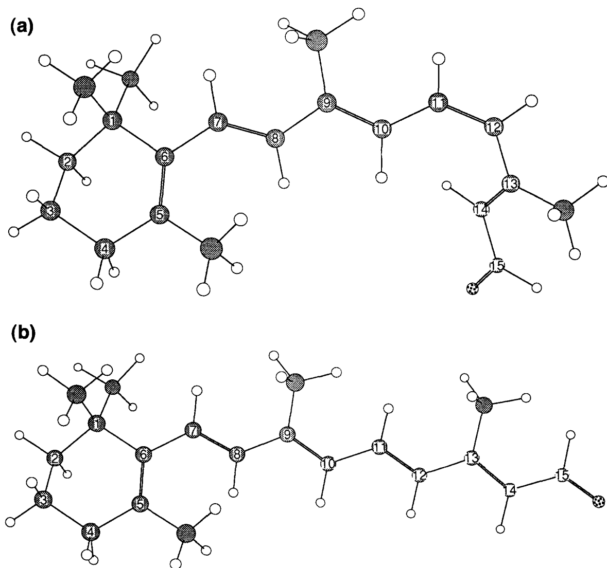
Fig. 1. Structures of the (a) 11-cis and (b) all-trans-retinal, showing the numbering system used in this Letter.
