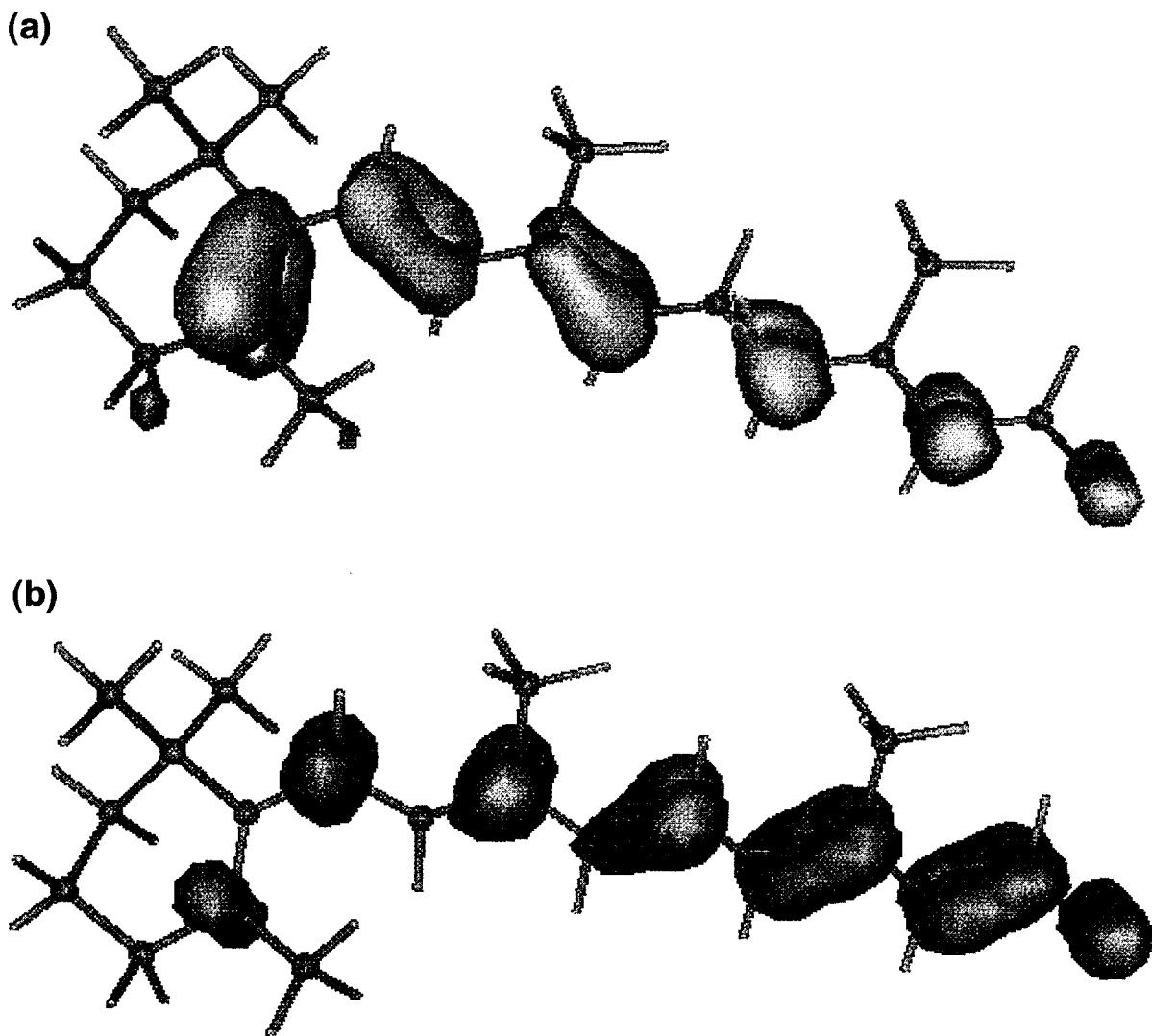
Fig. 2. HOMO (a) and LUMO (b) electron charge density distribution in all-trans-retinal. The isosurfaces shown in the pictures correspond to an electron density of 0.005 \text{ e}/\text{au}^3 and delimit a total electronic charge of about 1 electron.
