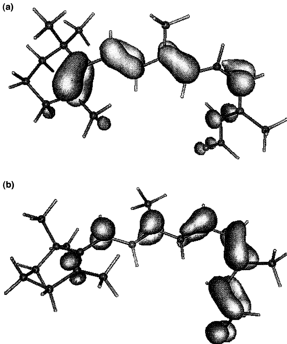
Fig. 3. HOMO (a) and LUMO (b) electron charge density distribution for 11-cis-retinal. Same visualization criteria as in Fig. 2.
