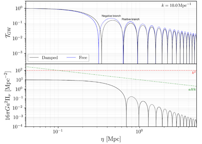
Figure 1. A figure showing an example of the neutrino damping term and its effect on the transfer function at k = 10 \text{ Mpc}^{-1} . The top panel reveals small phase shifts accompany a drop in amplitude of \mathcal{T}_{\text{GW}} around the time of horizon crossing. Dashed lines indicate negative branches of the oscillating function. The lower panel shows the damping term 16\pi G a^2 \Pi_\nu . Dotted lines show other terms in the differential equation associated with the wavenumber and Hubble expansion.
