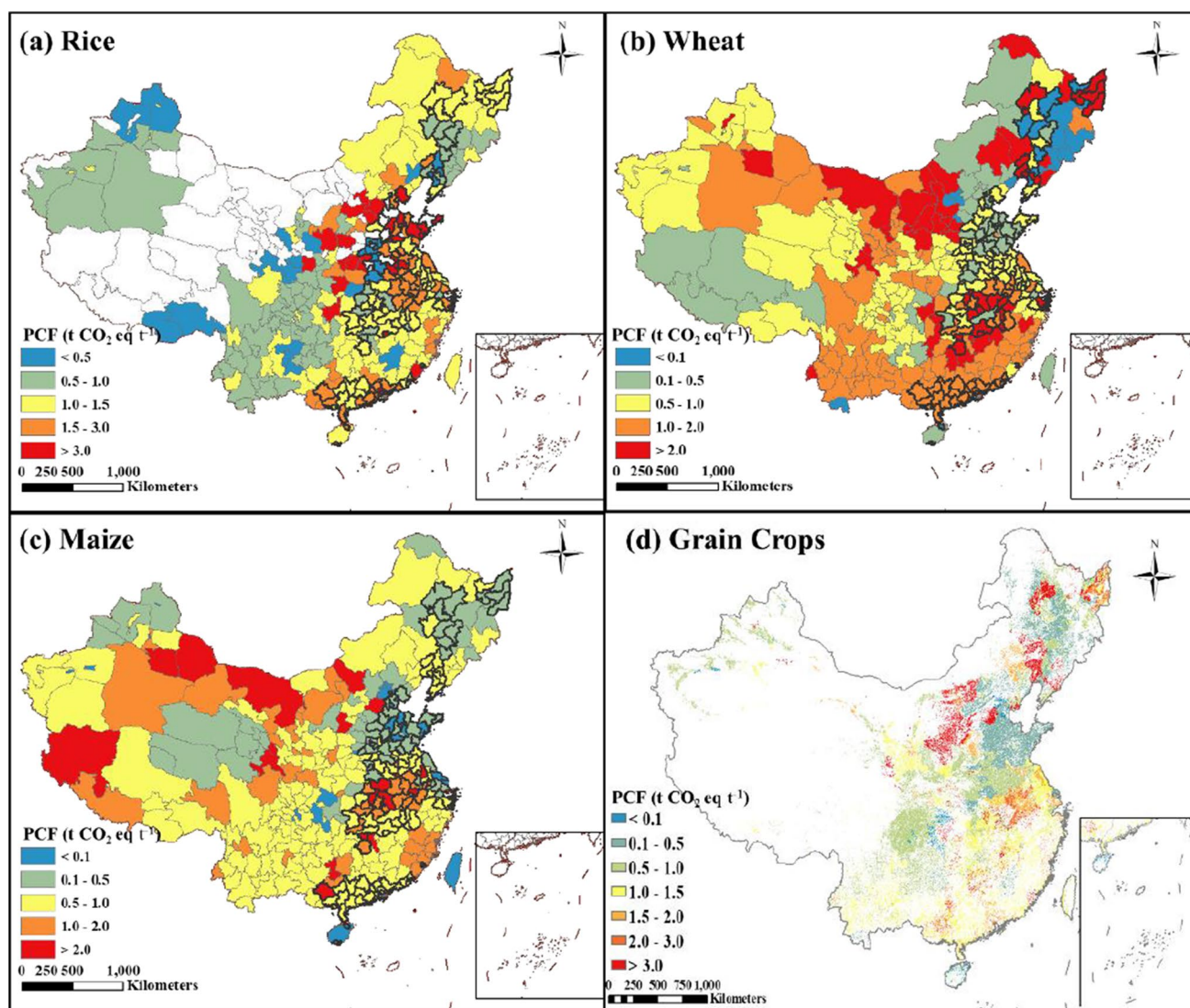
Fig. 5 PCFs of main grains production in 2015. a Rice. b Wheat. c Maize. d The spatial distribution of PCFs of three grains
