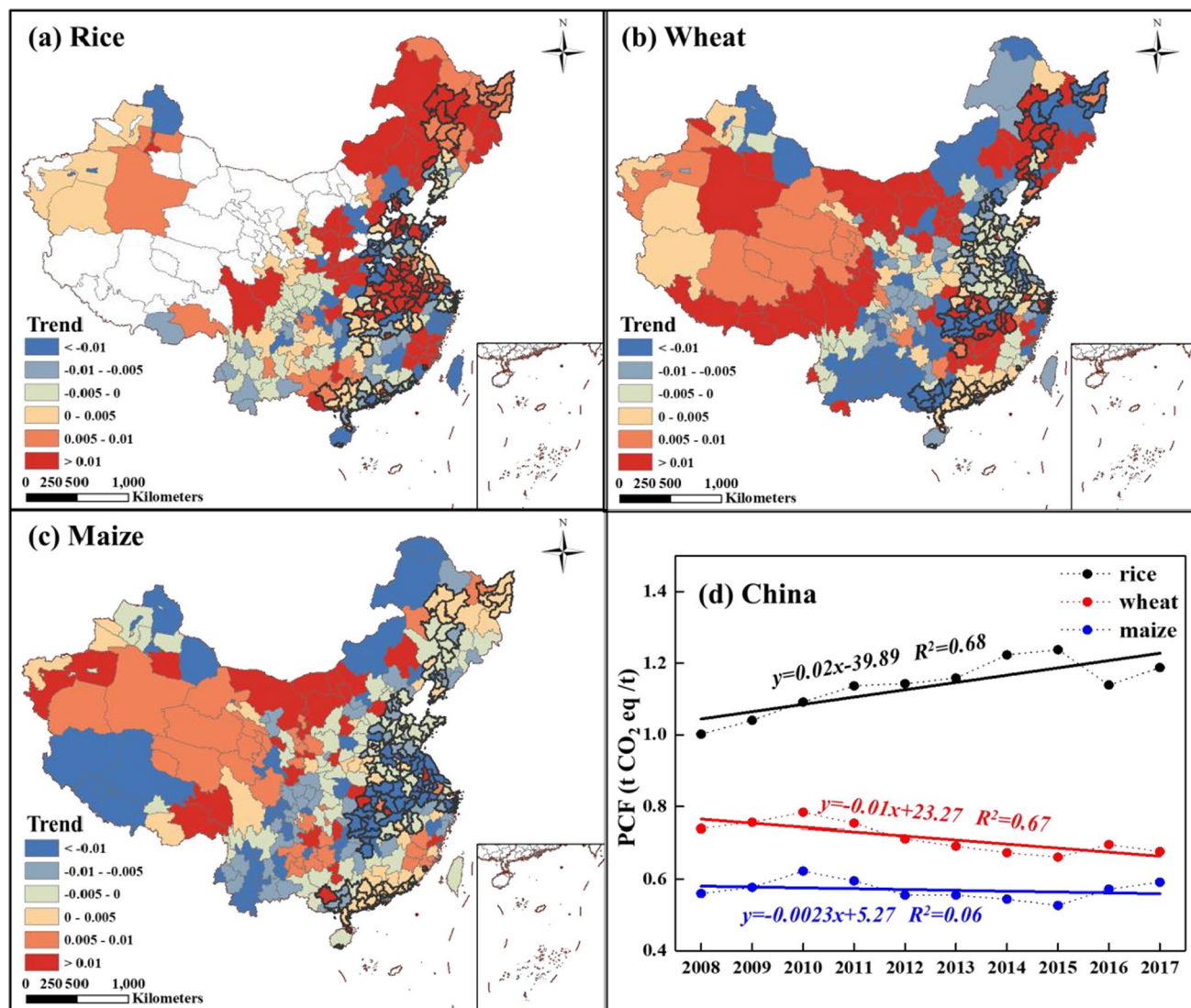
Fig. 7 Trends of PCFs from 2008 to 2017. a Rice. b Wheat. c Maize. d General tendency
