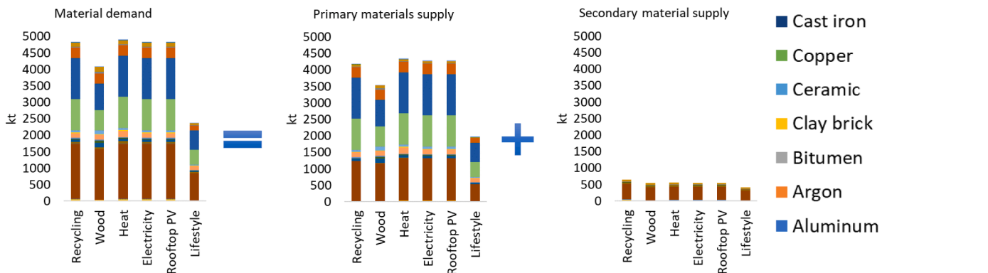
Fig. 3. Cumulative material demand and supply. The material demand is supplied by primary and secondary materials. The amounts of materials in Fig. 3c are the sums of material flows in the 2016–2050 period.
