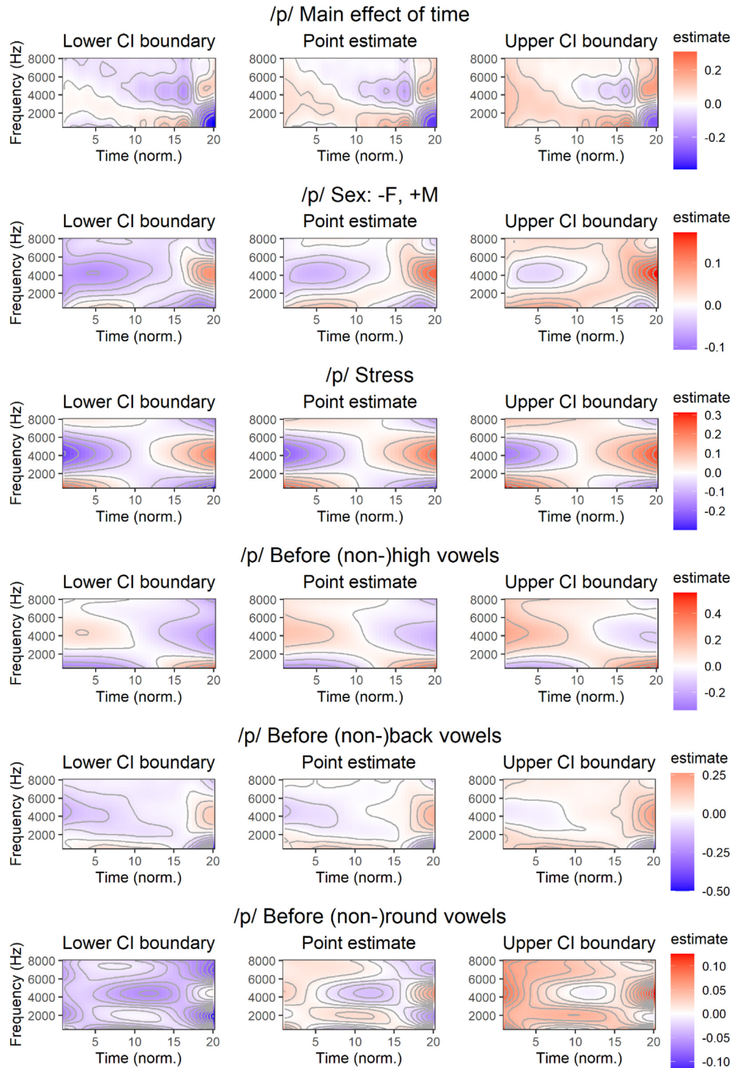
Appendix B.3. 95% confidence intervals of two-dimensional variables in the model of /p/ releases.
