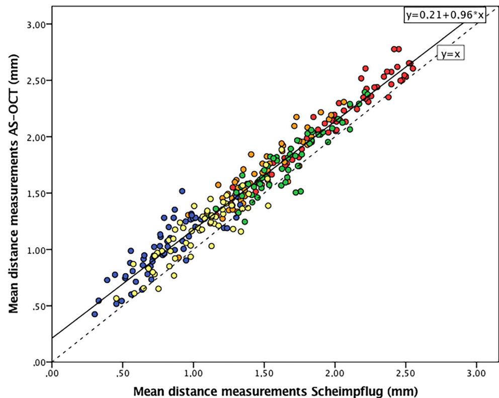
Fig. 3 Scatter plot of the anterior segment optical coherence tomography (AS-OCT) measurements against Scheimpflug imaging measurements. The regression fit line (black line) following the relationship of the devices consistently shows higher measurements of AS-OCT compared with the dashed line which represents the absolute agreement of the instruments. Dot colors represent the positions of distances from the pIOL to the endothelium: red: central; green: 2.5 mm temporal from the center; orange: 2.5 mm nasal from the center; yellow: 4.0 mm nasal from the center; blue: 4.0 mm nasal from the center
