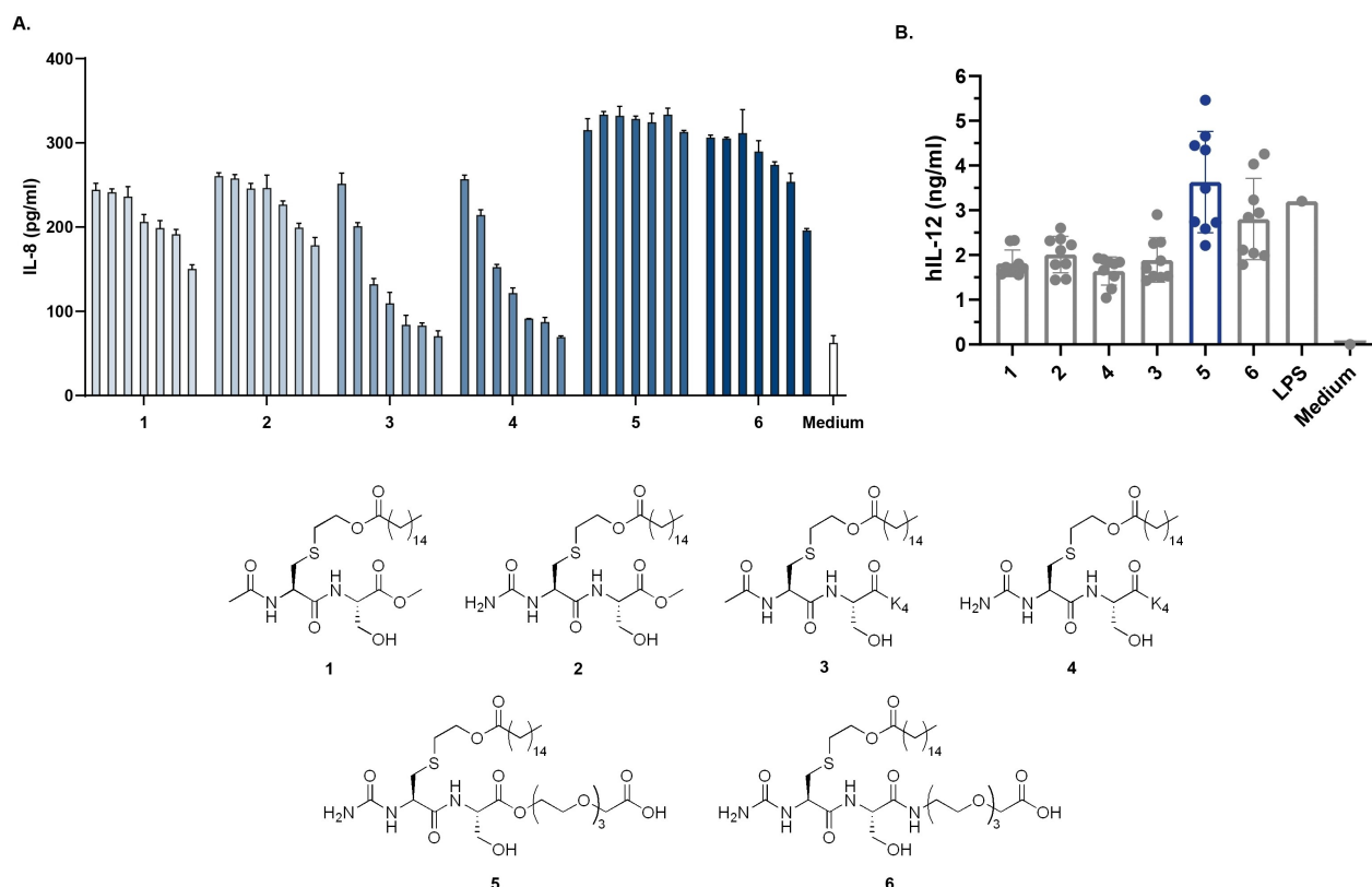
Figure 2. TLR2 activation of the different mini-UPam derivatives in A) HEK-TLR2 cells and B) human moDCs. Cells were incubated with titrated amounts (1 \mu\text{M} –15.6 nM and 1 \mu\text{M} –3.9 nM respectively, twofold titrations) of the indicated compounds (Scheme 1). The lipopolysaccharide (LPS) concentration was 1 \mu\text{g}/\text{mL} . After 36 h, supernatants were harvested, and the production of A) IL-8 (data shown as mean \pm SD, n=3 ) or B) IL-12p40 (data shown as mean \pm SD, n=9 ) was determined by specific ELISA.
