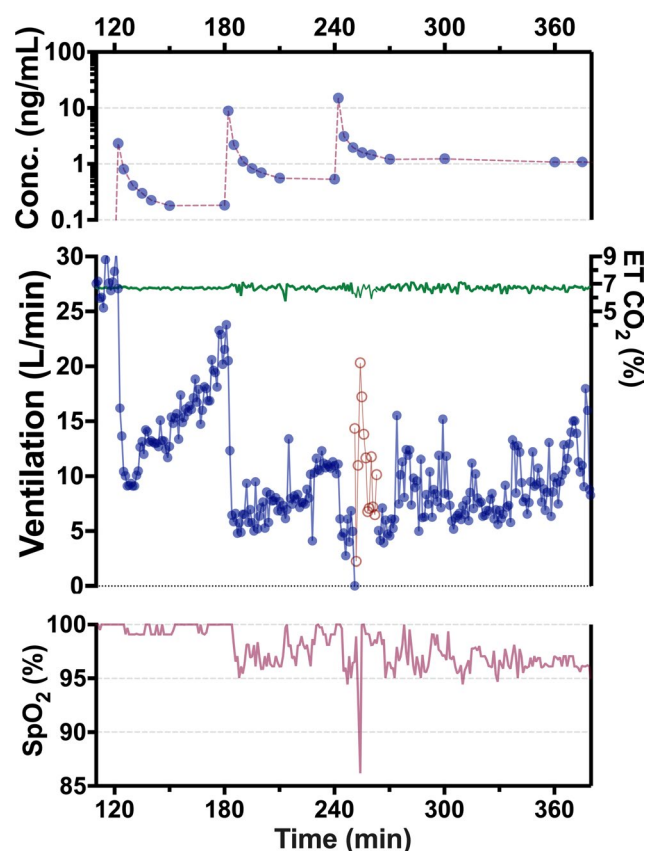
Figure 1 Example of effect of three fentanyl administrations (75 µg/70 kg, 150 µg/70 kg, and 250 µg/70 kg) on isohypercapnic ventilation in an opioid-naïve individual (subject #110). Top panel: The measured fentanyl plasma concentrations (Conc.). Middle panel: 1-minute ventilation averages (blue symbols = spontaneous breathing, red symbols = stimulated breathing during a 12-minute apneic period following the third fentanyl administration) and end-tidal CO 2 concentration (green line); bottom panel: oxygen saturation (SpO 2 ).
